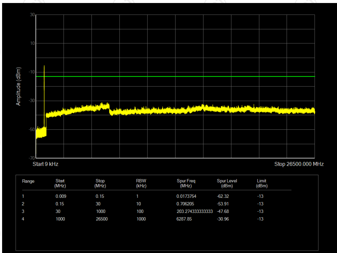
Band5 QPSK BW=1.4MHz Channel=20407 RB Size=6 Position=#0
