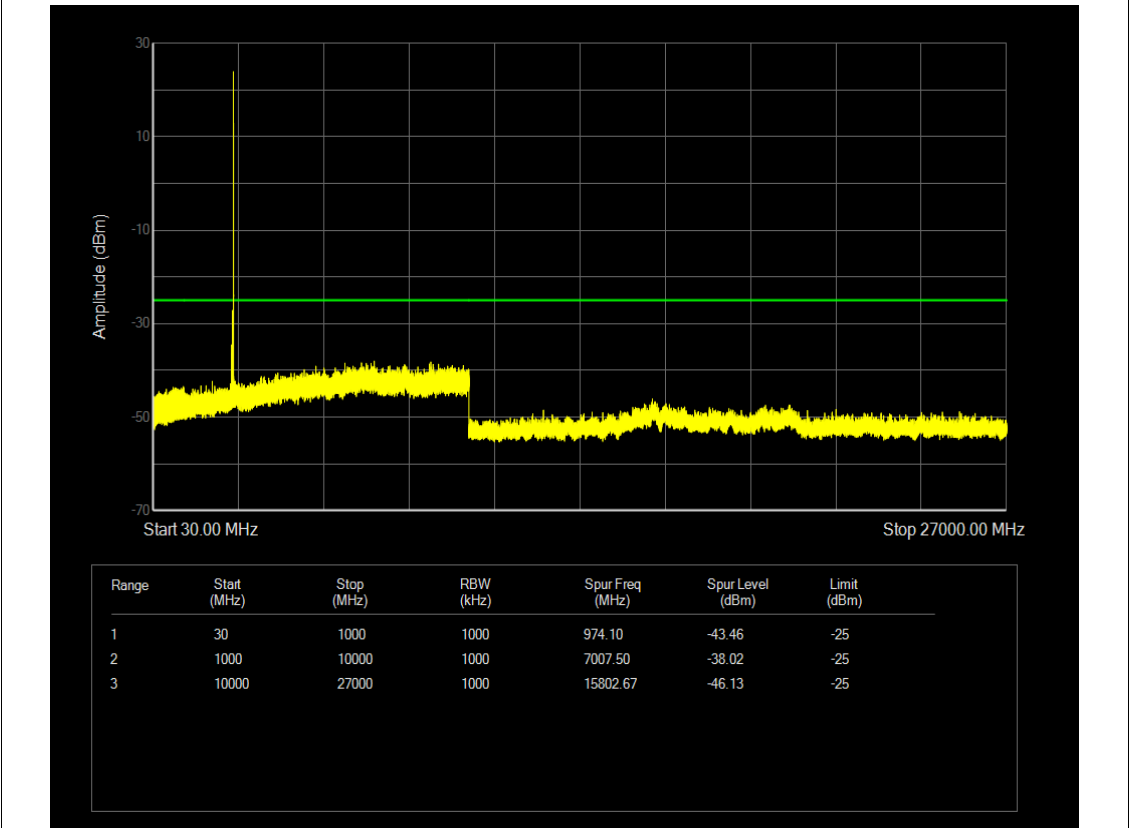
n41 SCS=30kHz DFT_BPSK BW=60MHz Channel=505200 RB=1@161
