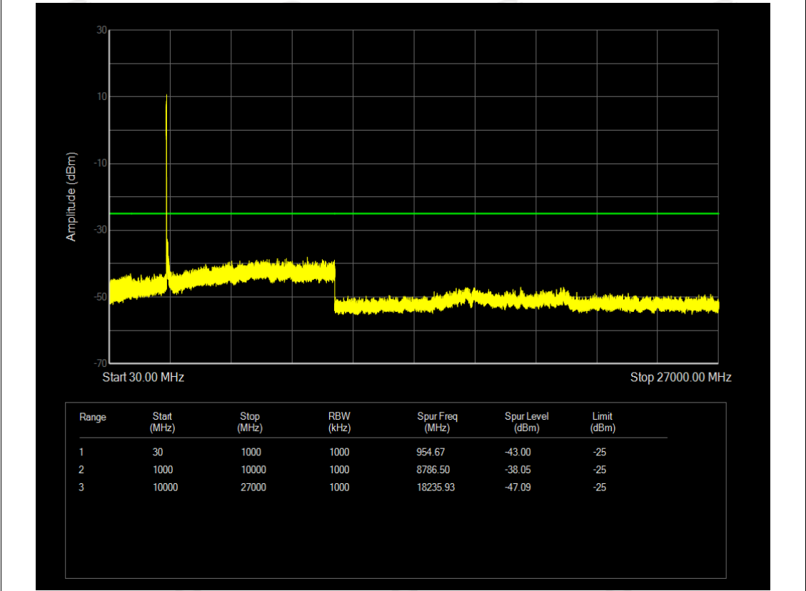
n41 SCS=30kHz DFT_BPSK BW=60MHz Channel=505200 RB=162@0
