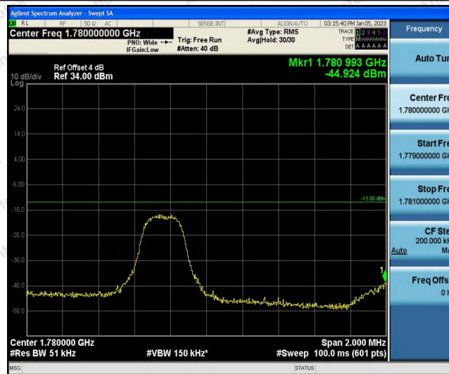
Band66-3MHz-16QAM-132657-1RB#14
