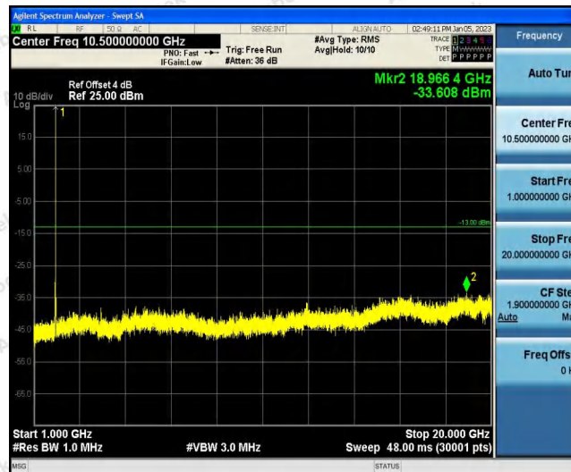
Band25-20MHz-16QAM-26590-1RB#0-Range2:1000~20000MHz
