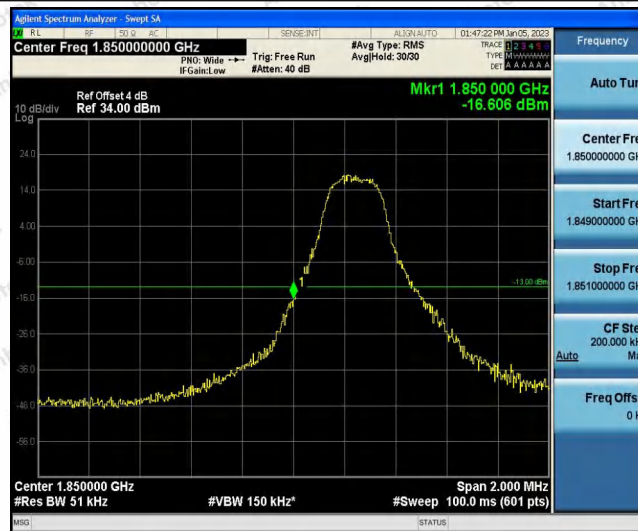
Band25-3MHz-16QAM-26055-1RB#14
