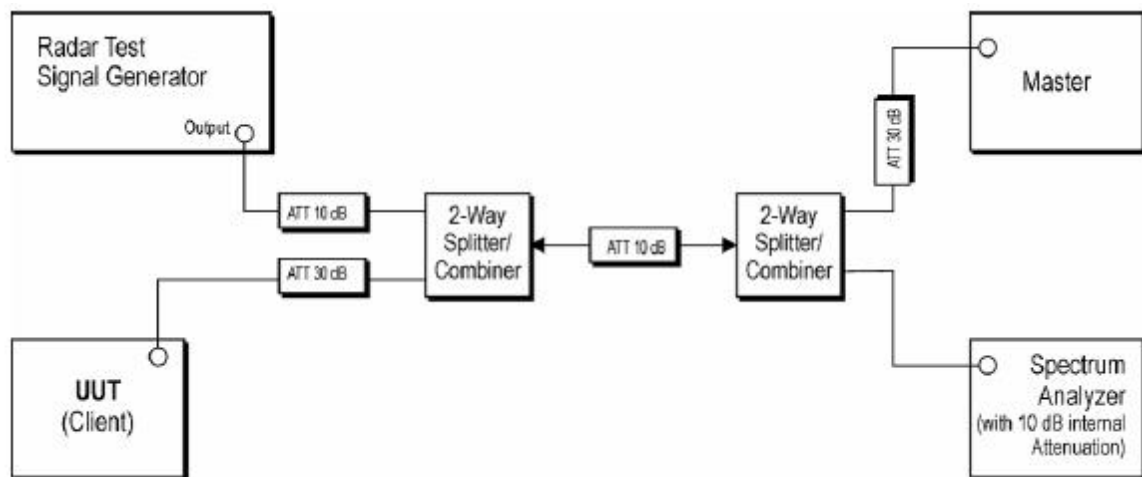
Example Conducted Setup where UUT is a Client and Radar Test Waveforms are injected into the Master
