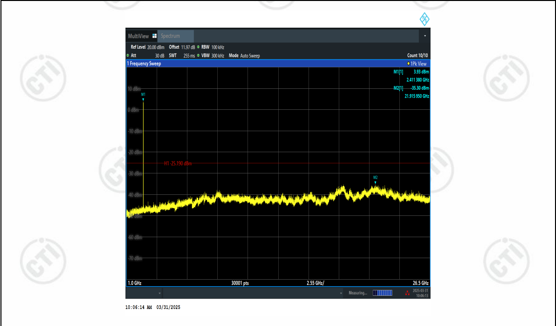
11B-Ant2-2412-1000~26500-PASS
