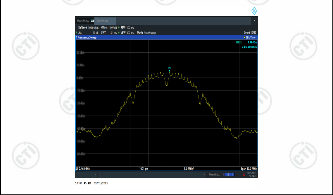
11B-Ant2-2462-0~Reference-PASS
