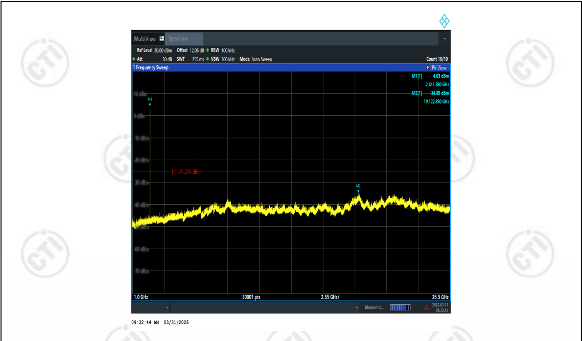
11B-Ant1-2412-1000~26500-PASS
