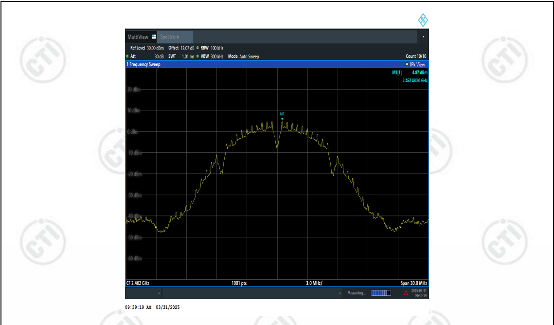
11B-Ant1-2462-0~Reference-PASS
