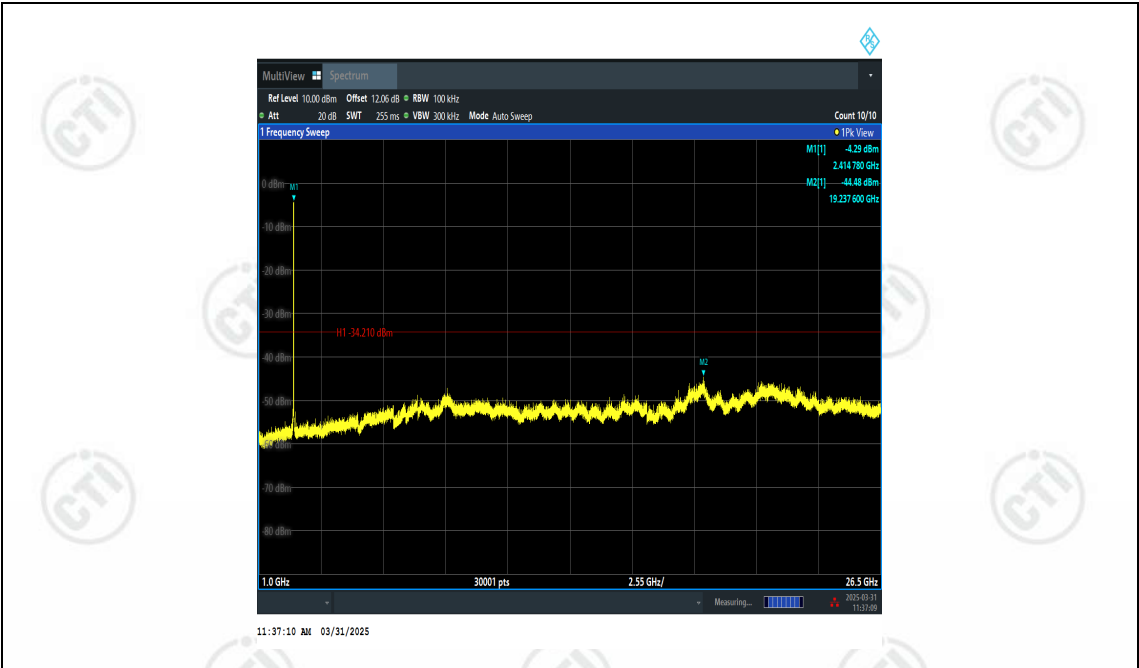
11N20MIMO-Ant1-2412-1000~26500-PASS
