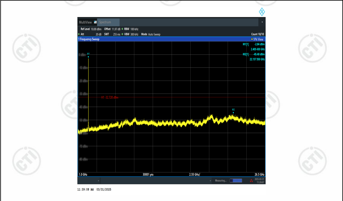
11N20MIMO-Ant2-2412-1000~26500-PASS
