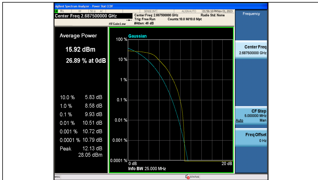
Band41-5MHz-QPSK-41565-25RB#0-PASS
