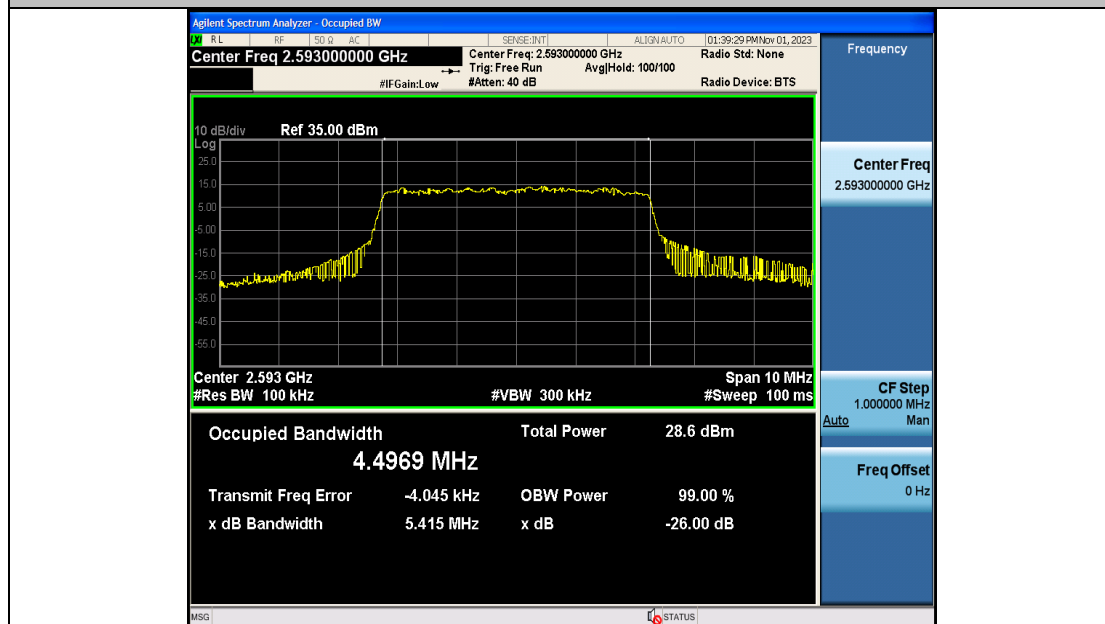
Band41-5MHz-16QAM-40620-25RB#0-PASS
