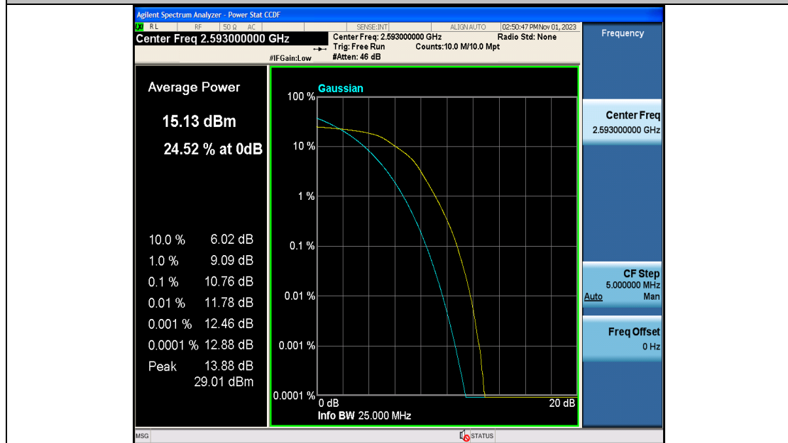
Band41-20MHz-16QAM-40620-100RB#0-PASS
