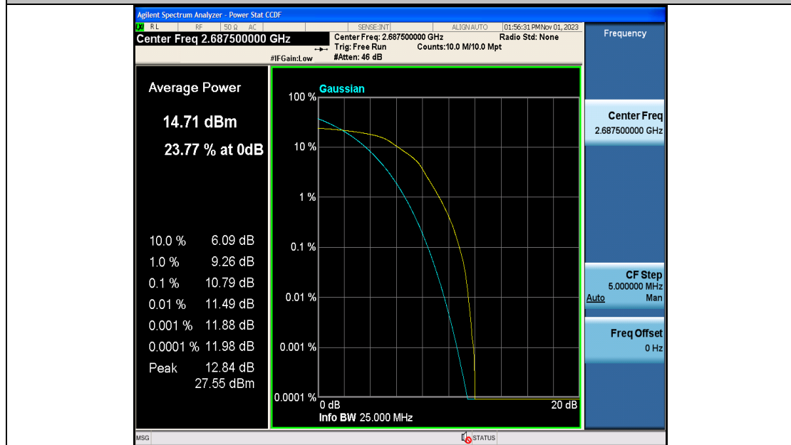
Band41-5MHz-16QAM-41565-25RB#0-PASS
