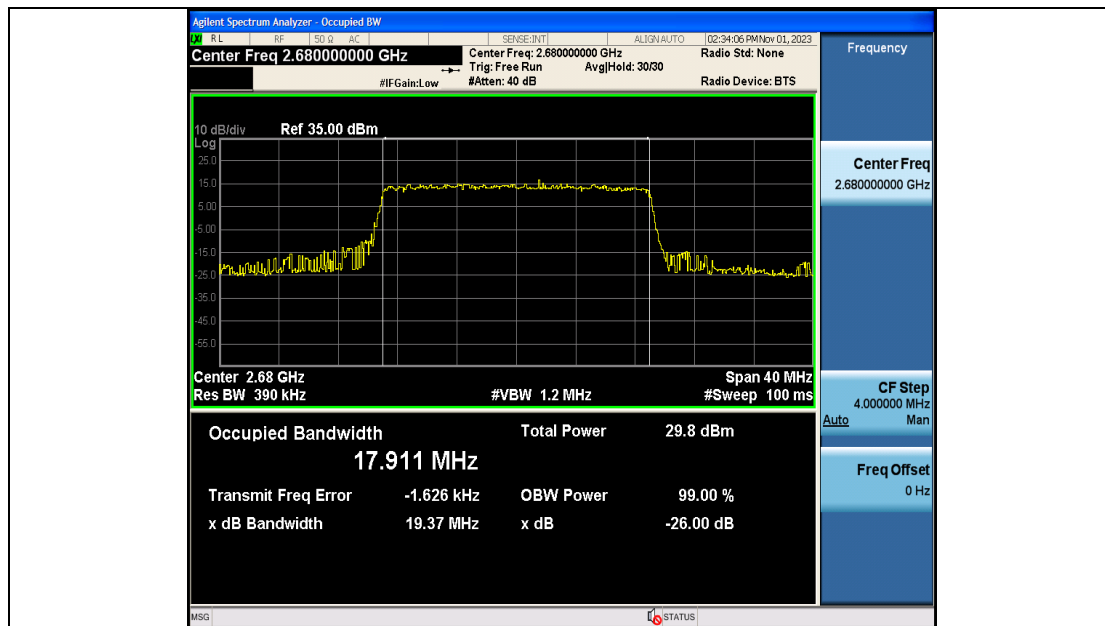
Band41-20MHz-QPSK-41490-100RB#0-PASS
