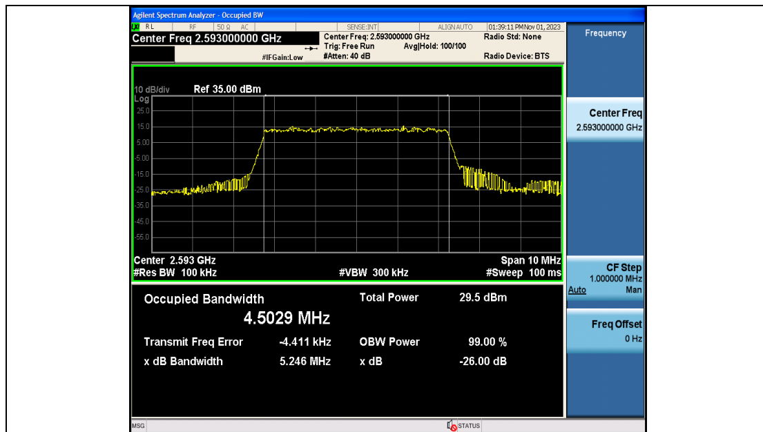
Band41-5MHz-QPSK-40620-25RB#0-PASS
