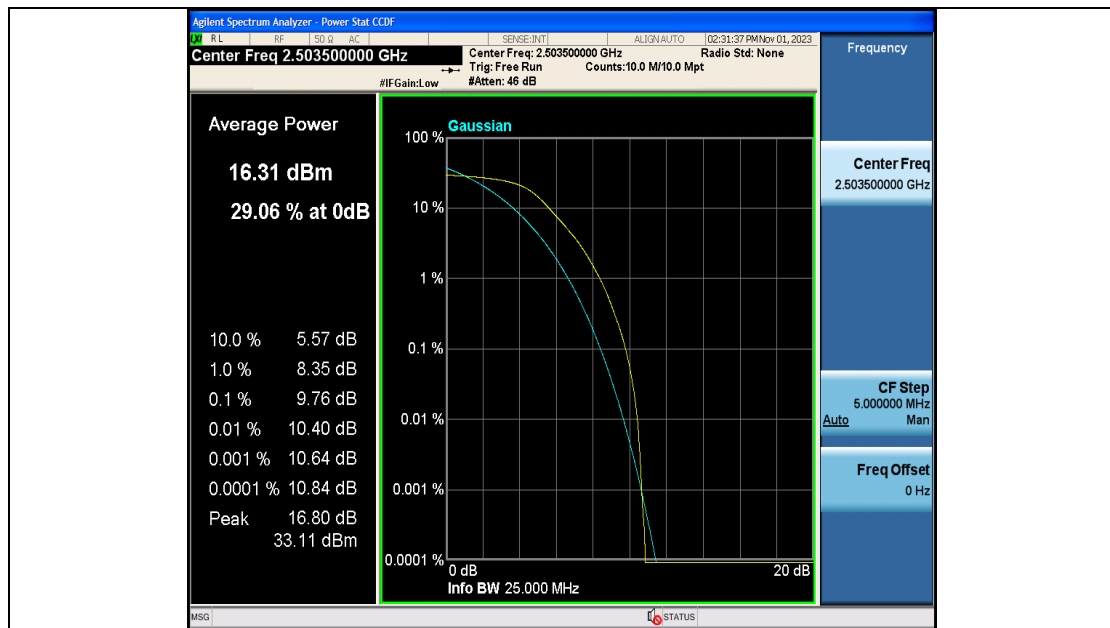
Band41-15MHz-QPSK-39725-75RB#0-PASS
