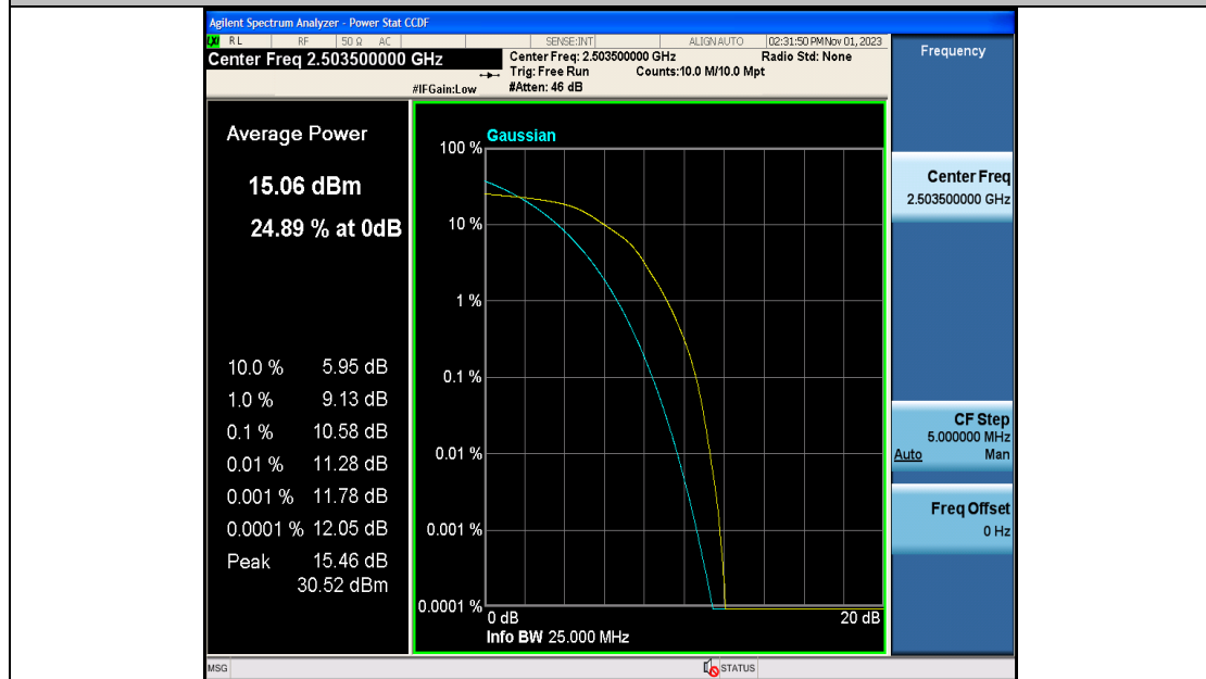
Band41-15MHz-16QAM-39725-75RB#0-PASS
