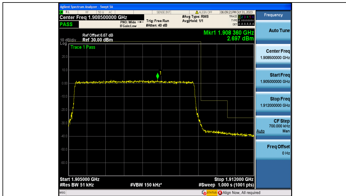
Band2_5MHz_QPSK_19175_25RB#0
