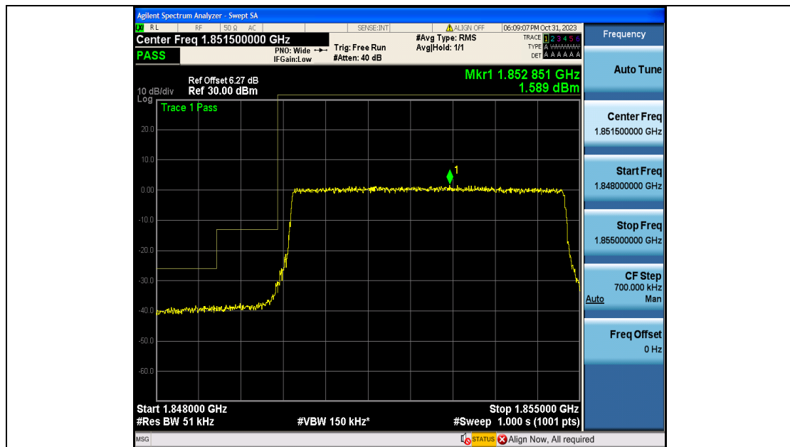
Band2_5MHz_QPSK_18625_25RB#0
