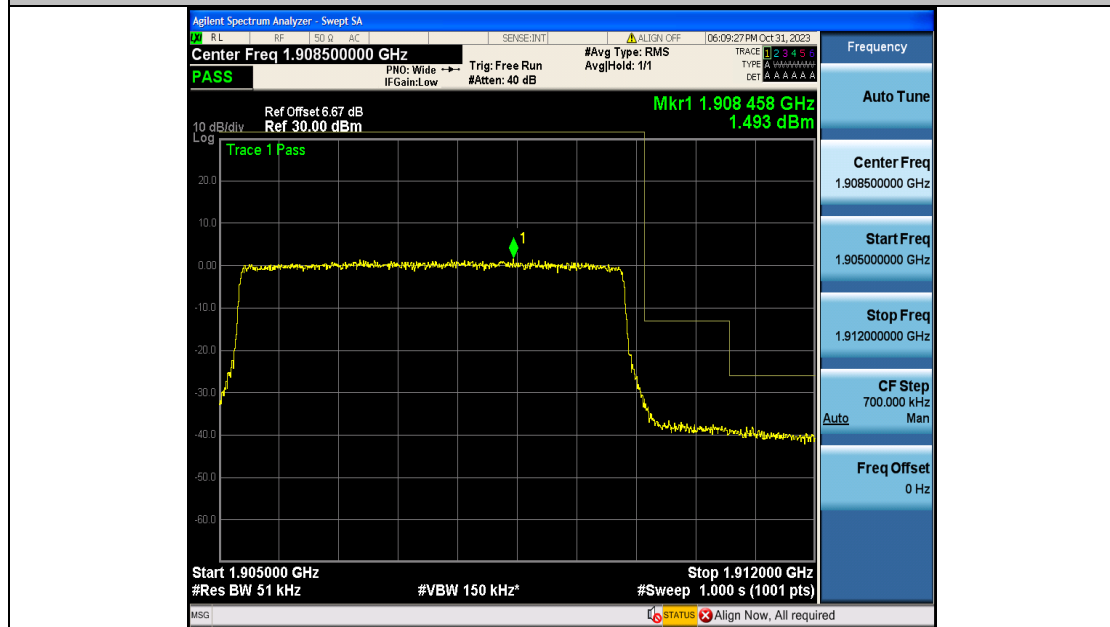
Band2_5MHz_16QAM_19175_25RB#0
