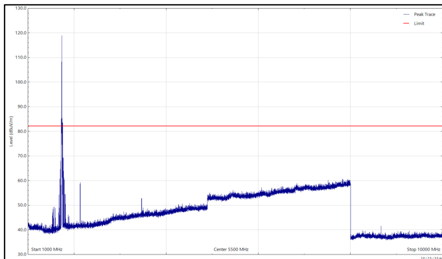
Figure 3 - LTE Cat M1_FDD Band 4_QPSK_BW 1.4 MHz_1747.5 MHz, 1 GHz to 10 GHz, Horizontal (Peak)
