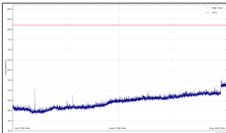
Figure 7 - LTE Cat M1_FDD Band 12_QPSK_BW 1.4 MHz_707.5 MHz, 1 GHz to 5 GHz, Horizontal (Peak)
