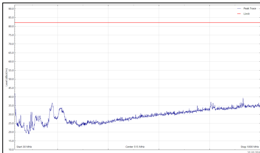
Figure 2 - LTE Cat M1_FDD Band 4_QPSK_BW 1.4 MHz_1747.5 MHz, 30 MHz to 1 GHz, Horizontal (Peak)
