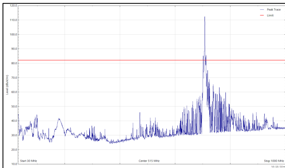
Figure 6 - LTE Cat M1_FDD Band 12_QPSK_BW 1.4 MHz_707.5 MHz, 30 MHz to 1 GHz, Horizontal (Peak)
