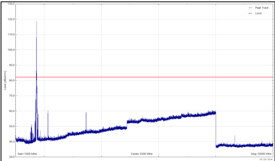
Figure 5 - LTE Cat M1_FDD Band 4_QPSK_BW 1.4 MHz_1747.5 MHz, 1 GHz to 10 GHz, Vertical (Peak)
