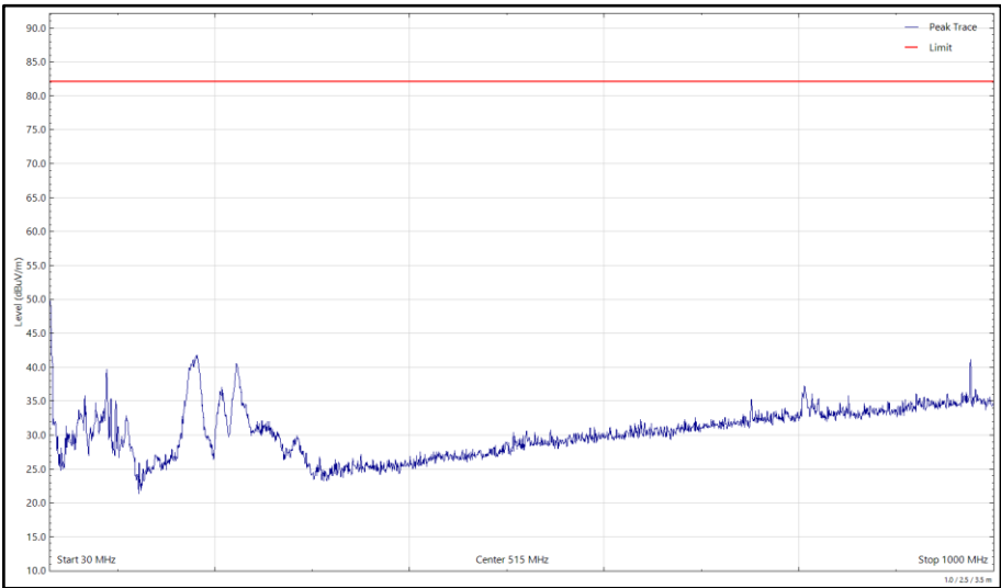
Figure 4 - LTE Cat M1_FDD Band 4_QPSK_BW 1.4 MHz_1747.5 MHz, 30 MHz to 1 GHz, Vertical (Peak)
