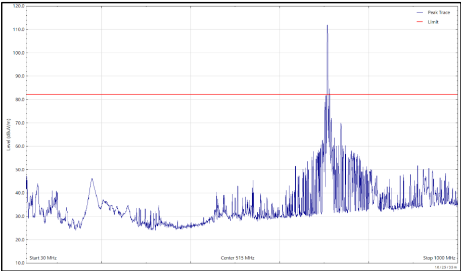
Figure 8 -LTE Cat M1_FDD Band 12_QPSK_BW 1.4 MHz_707.5 MHz, 30 MHz to 1 GHz, Vertical (Peak)
