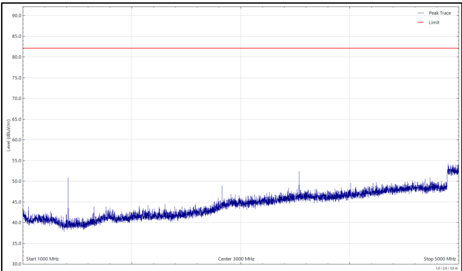
Figure 9 - LTE Cat M1_FDD Band 12_QPSK_BW 1.4 MHz_707.5 MHz, 1 GHz to 5 GHz, Vertical (Peak)
