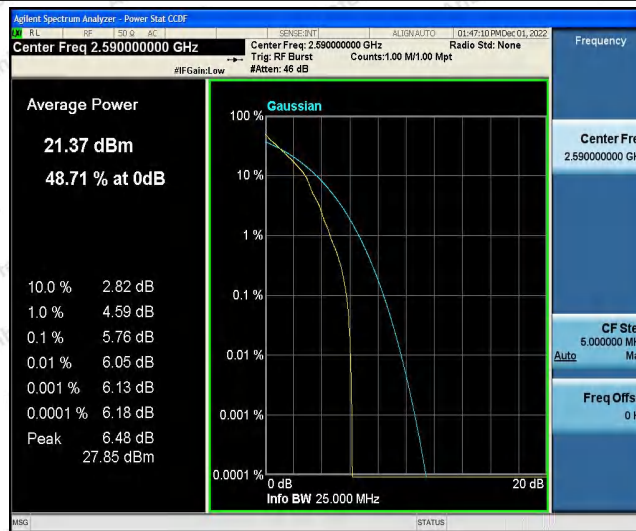
Band41-10MHz-QPSK-40590-50RB#0
