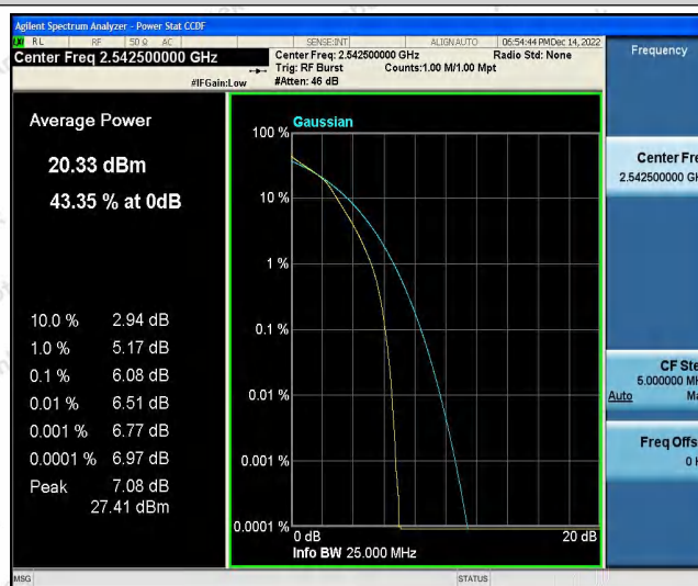
Band41-15MHz-16QAM-40590-1RB#0
