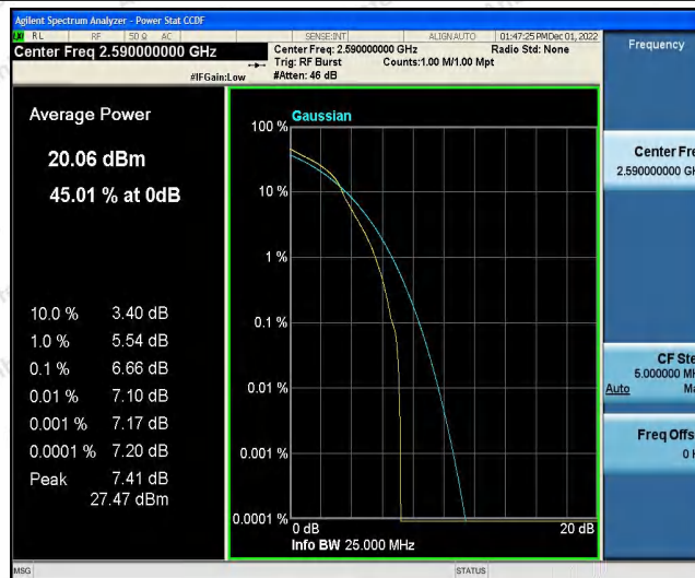
Band41-10MHz-16QAM-40590-50RB#0
