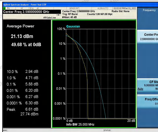
Band41-15MHz-QPSK-40590-75RB#0
