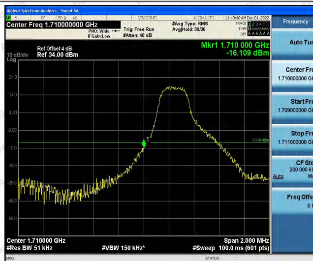
Band66-3MHz-16QAM-131987-1RB#14
