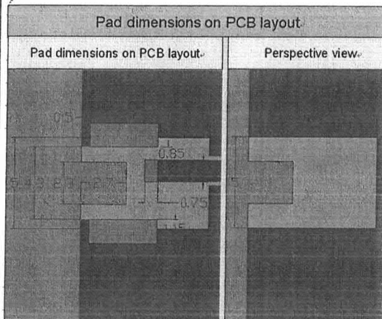
PCB pad dimensions
