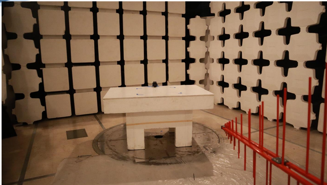
30MHz-1GHz Radiated Emissions
