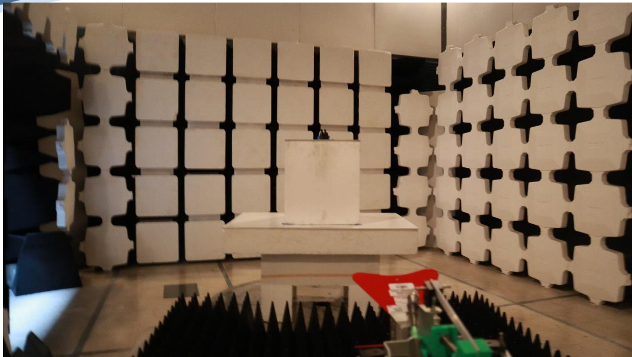
Tx Spurious above 1GHz
