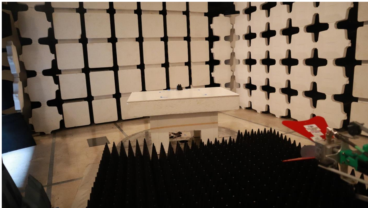
1-18GHz Radiated Emissions
