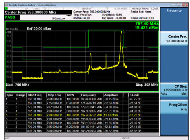
FDD14-10MHz-16QAM-MCH-1RB#49
