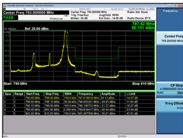
FDD14-5MHz-QPSK-HCH-1RB#24
