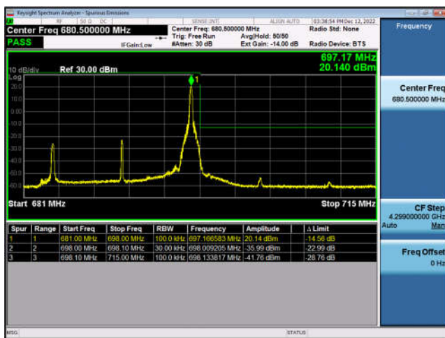
FDD71-15MHz-QPSK-HCH-75RB#0
