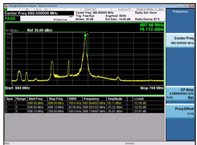
FDD71-5MHz-16QAM-HCH-1RB#24
