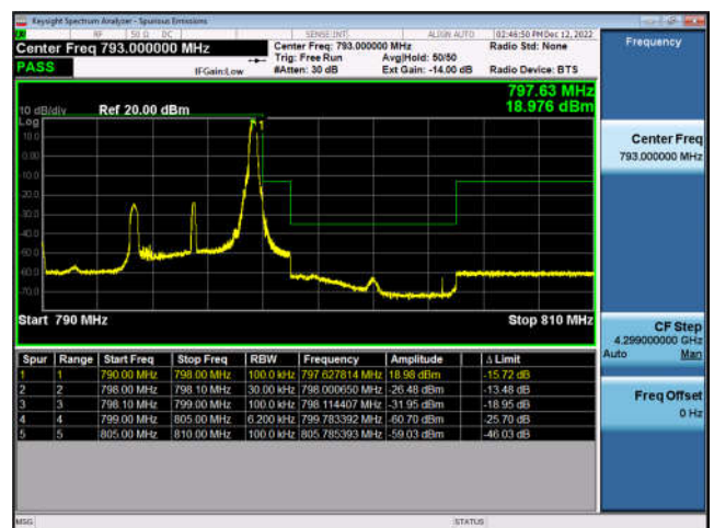
FDD14-5MHz-16QAM-HCH-1RB#24
