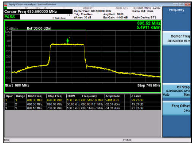
FDD71-10MHz-16QAM-LCH-1RB#0
