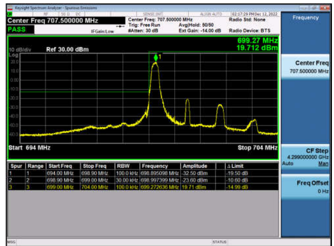
FDD12-3MHz-16QAM-LCH-15RB#0
