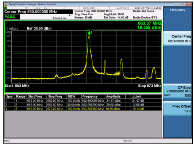
FDD71-5MHz-16QAM-LCH-25RB#0
