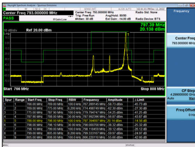
FDD14-10MHz-QPSK-MCH-1RB#49
