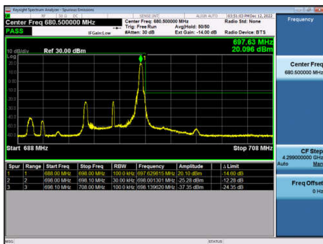
FDD71-5MHz-QPSK-HCH-1RB#24
