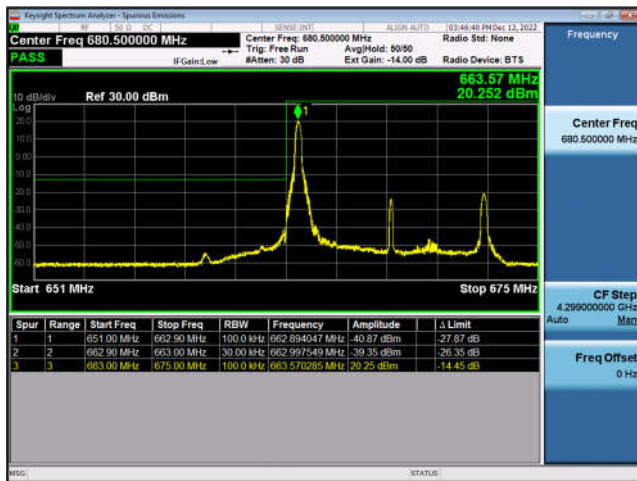
FDD71-10MHz-QPSK-LCH-50RB#0
