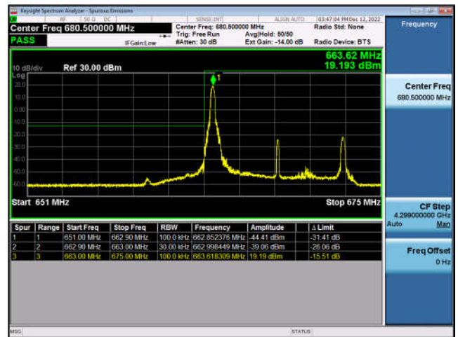
FDD71-10MHz-16QAM-LCH-50RB#0
