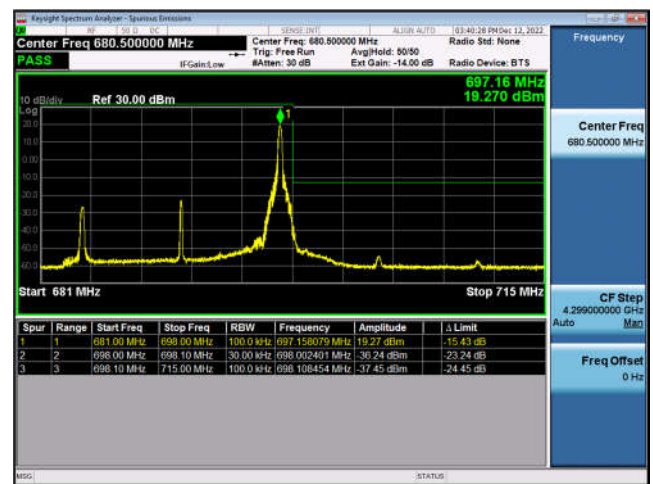
FDD71-15MHz-16QAM-HCH-75RB#0
