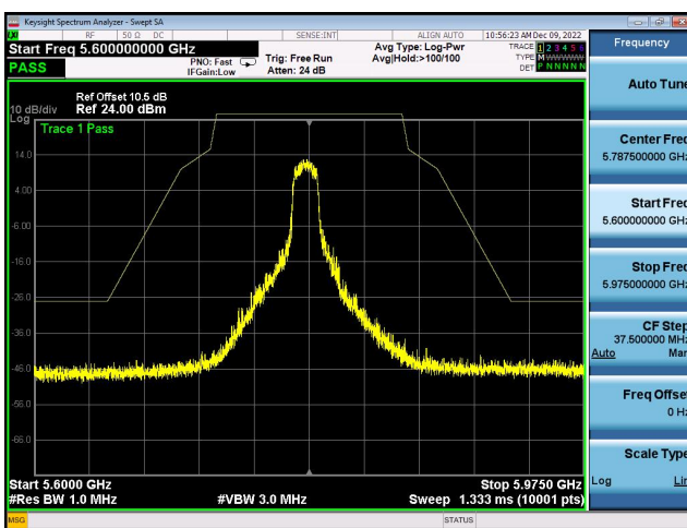
U-NII-3 ,Plot 1,Band Edge-802.11a(20MHz),5785MHz,Ant1
