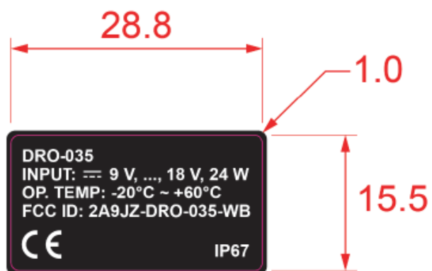
Figure 1 – [DRO-035-703] RfPatrol Mk2 WB SPEC Label
