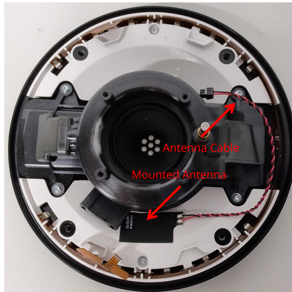
Exposed Antenna
