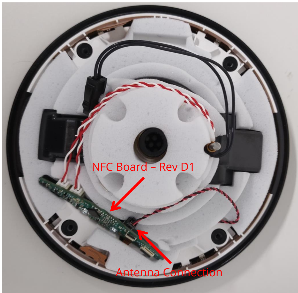
Complete Sub-Assembly
