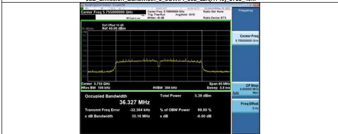
-6dB Emission Bandwidth 5_8WiFi 802_11n(HT40) 5755_40M
