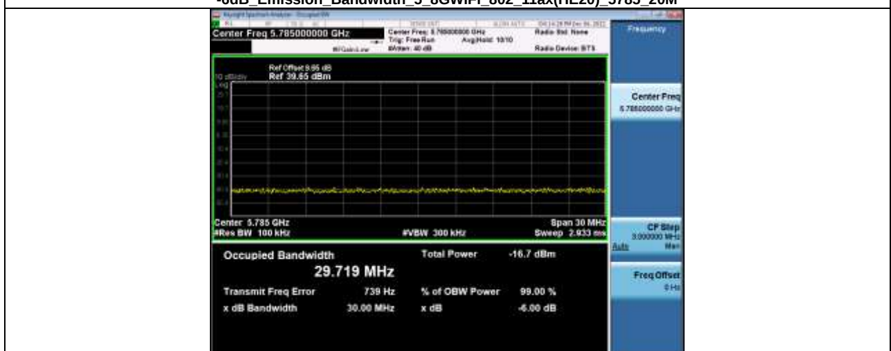
-6dB Emission Bandwidth 5 8WiFi 802 11ax(HE20) 5785 20M
