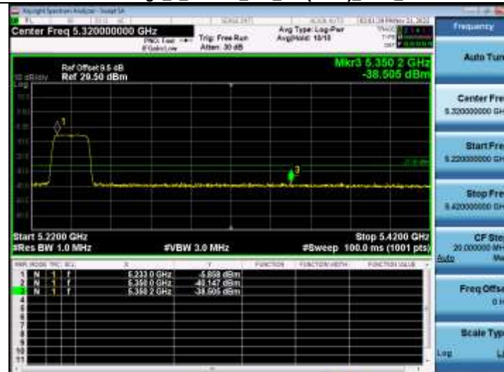
Bandedge_5_2GWiFi_802_11n(HT20)_5240_20M
