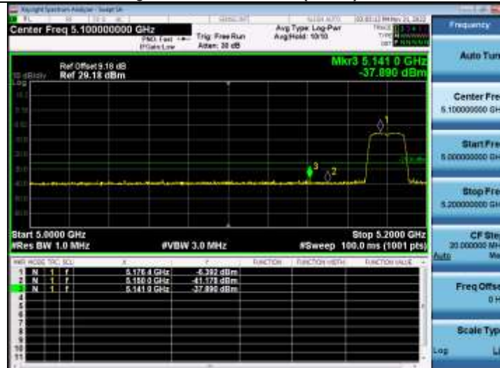
Bandedge_5_2GWiFi_802_11ac(VHT20)_5180_20M
