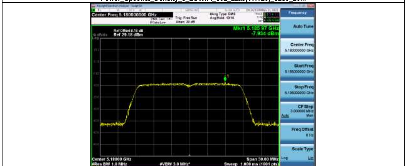
Power_Spectral_Density_5_2GWiFi_802_11ac(VHT20)_5180_20M
