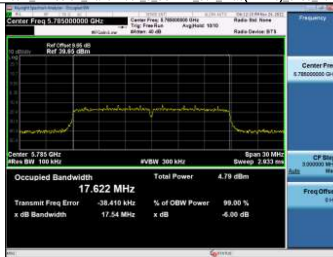
-6dB Emission Bandwidth 5.8GHz WiFi 802.11ac(VHT20) 5785_20M
