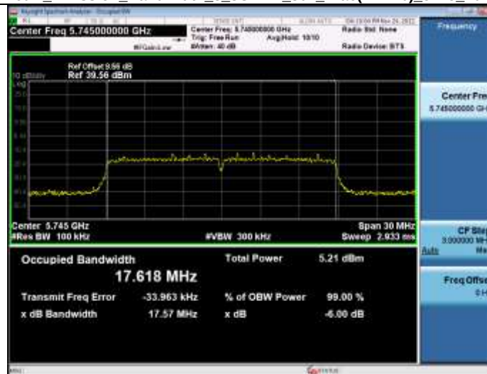
-6dB Emission Bandwidth 5.8GHz WiFi 802.11ac(VHT20) 5745_20M
