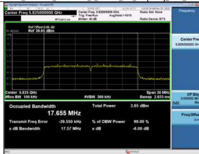
-6dB_Emission_Bandwidth_5_8WiFi_802_11n(HT20)_5825_20M
