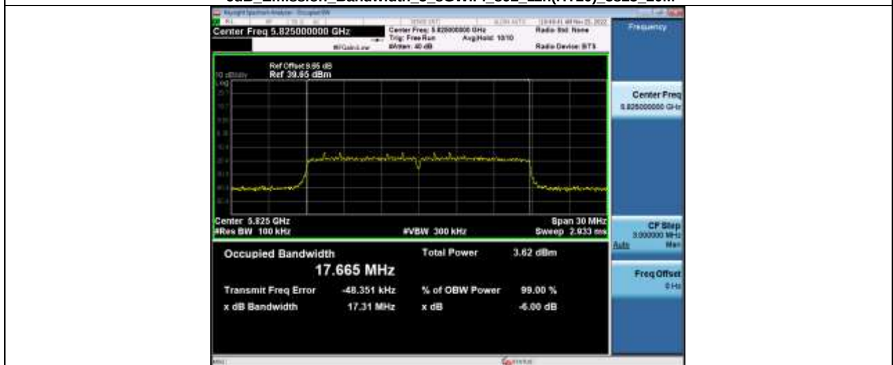
-6dB_Emission_Bandwidth_5_8WiFi_802_11n(HT20)_5825_20M
