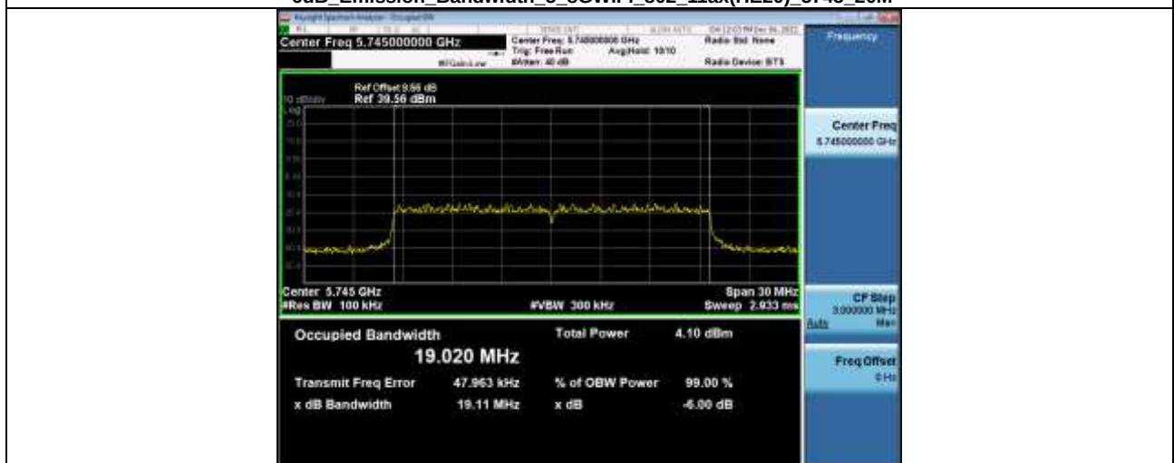
-6dB Emission Bandwidth 5 8WiFi 802 11ax(HE20) 5745 20M
