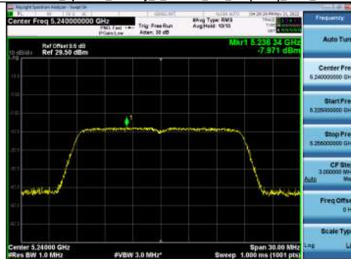
Power_Spectral_Density_5_2WiFi_802_11n(HT20)_5240_20M
