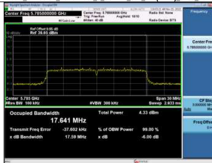
-6dB_Emission_Bandwidth_5_8WiFi_802_11n(HT20)_5785_20M
