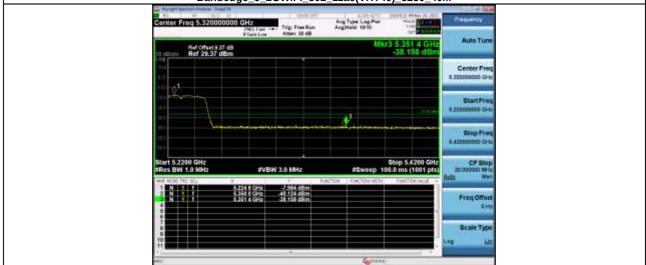
Bandedge_5_2GWiFi_802_11ac(VHT80)_5210_80M
