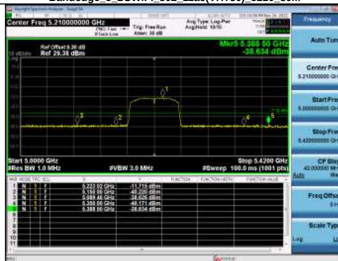
Bandedge 5 2GWiFi 802 11ac(VHT80) 5210 80M
