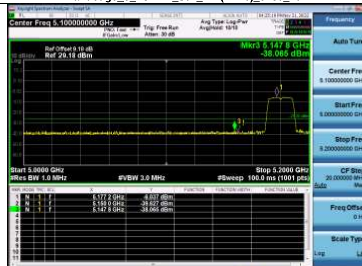
Bandedge 5_2GWiFi_802_11n(HT20)_5180_20M
