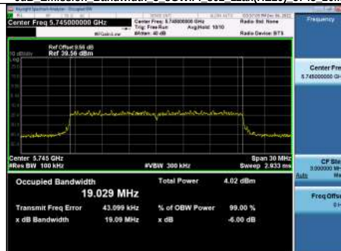
-6dB Emission Bandwidth 5_8WiFi 802_11ax(HE20)_5745_20M
