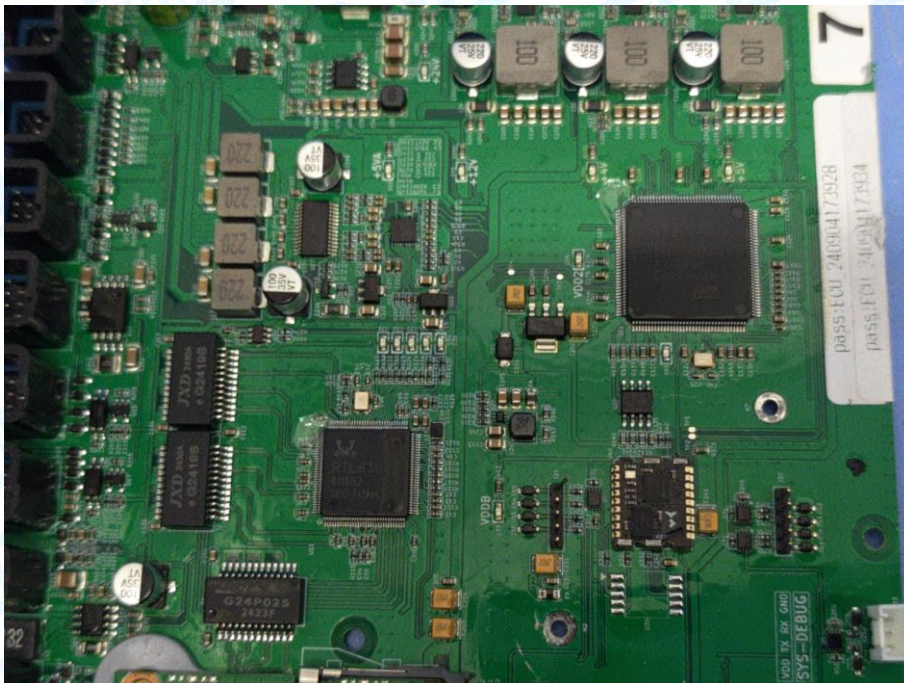
Photo 38 Appearance of PCB
