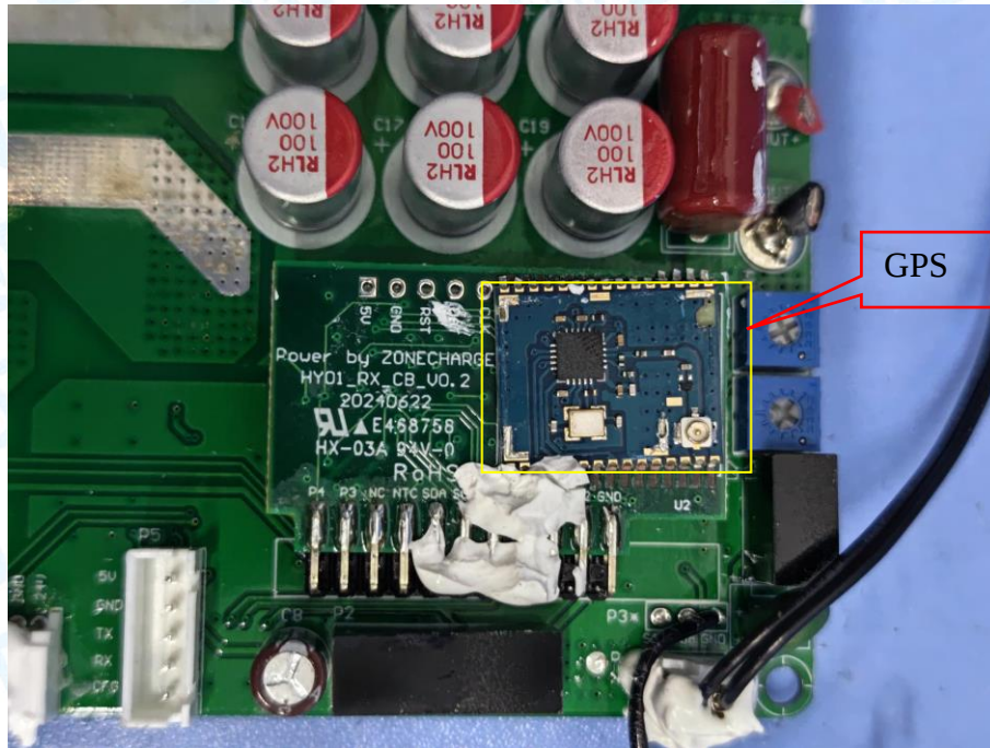
Photo 36 Appearance of PCB
