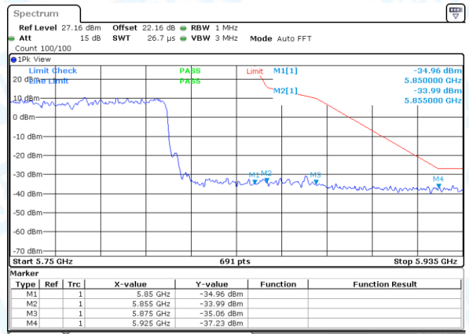
11AX80MIMO-Ant1-5775-PASS
