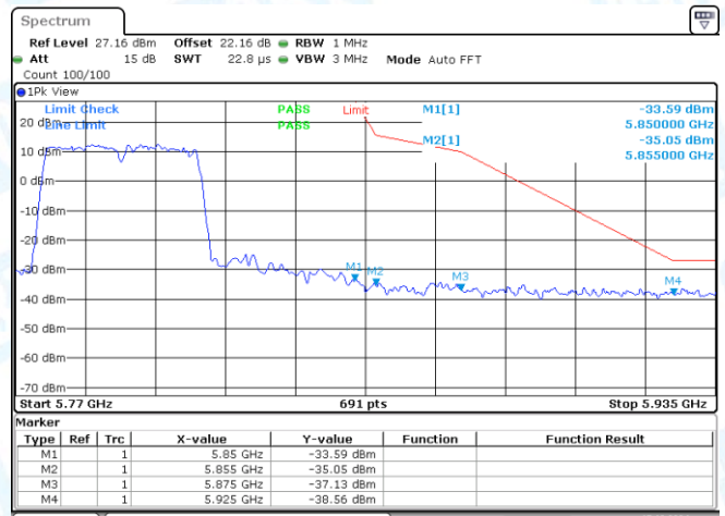
11N40MIMO-Ant2-5755-PASS
