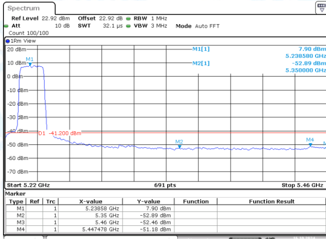
11N20MIMO-Ant1-5240-PASS
