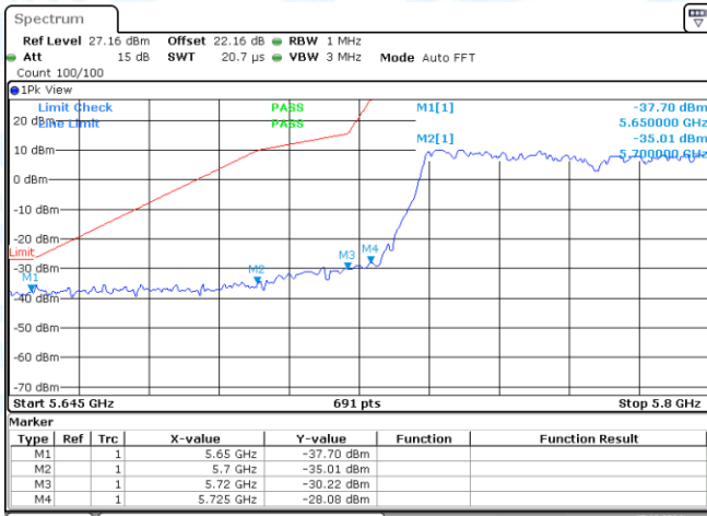
11AC80MIMO-Ant1-5775-PASS
