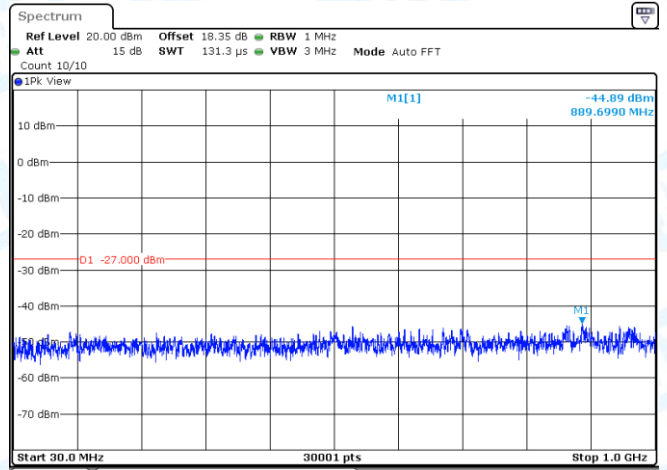
11AC20MIMO-Ant2-5825-30~1000-PASS
