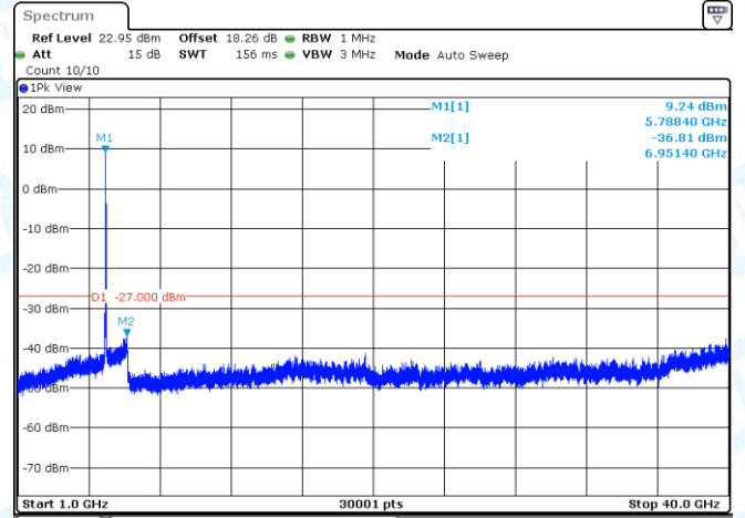
11AC40MIMO-Ant2-5795-1000~40000-PASS
