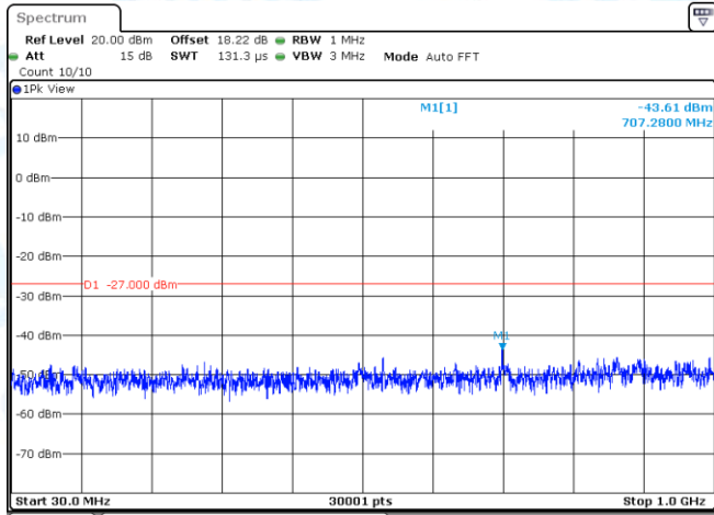
11AX80MIMO-Ant1-5775-30~1000-PASS
