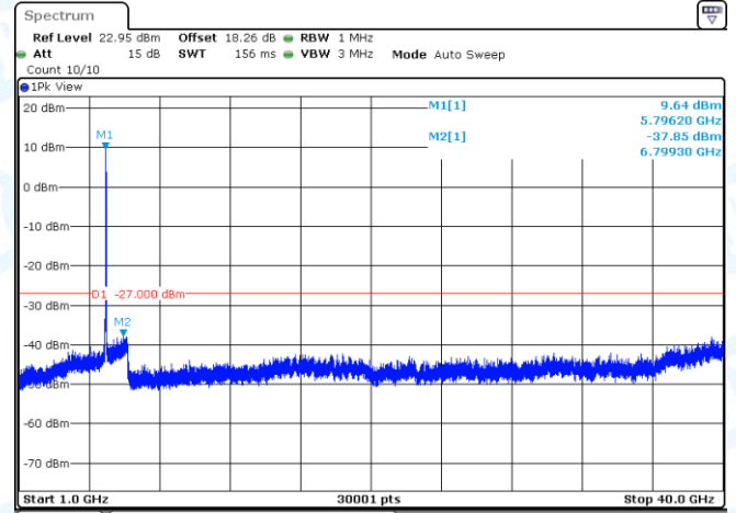
11AX40MIMO-Ant2-5795-1000~40000-PASS
