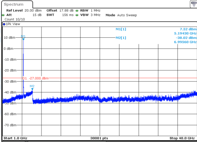
11AC40MIMO-Ant1-5190-1000~40000-PASS
