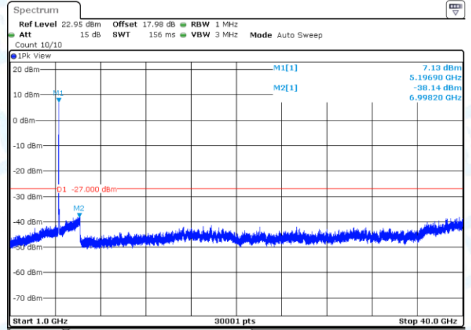
11AC40MIMO-Ant2-5190-1000~40000-PASS
