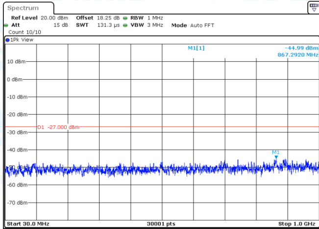
11AC40MIMO-Ant1-5755-30~1000-PASS
