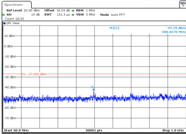
11AC20MIMO-Ant1-5825-30~1000-PASS
