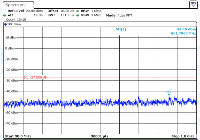
11AX80MIMO-Ant2-5775-30~1000-PASS
