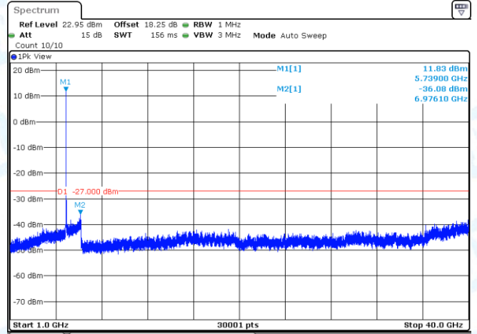
11AX20MIMO-Ant2-5745-1000~40000-PASS
