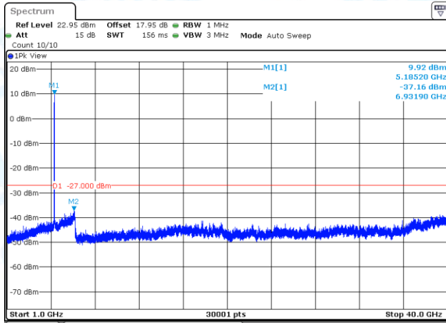
11AC20MIMO-Ant1-5180-1000~40000-PASS
