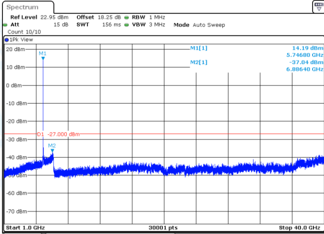
11AX20MIMO-Ant1-5745-1000~40000-PASS
