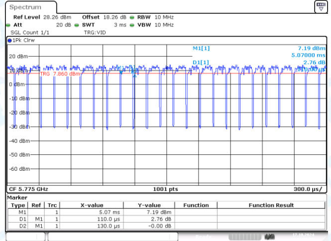
NTNV-11AX80MIMO-Ant2-5775
