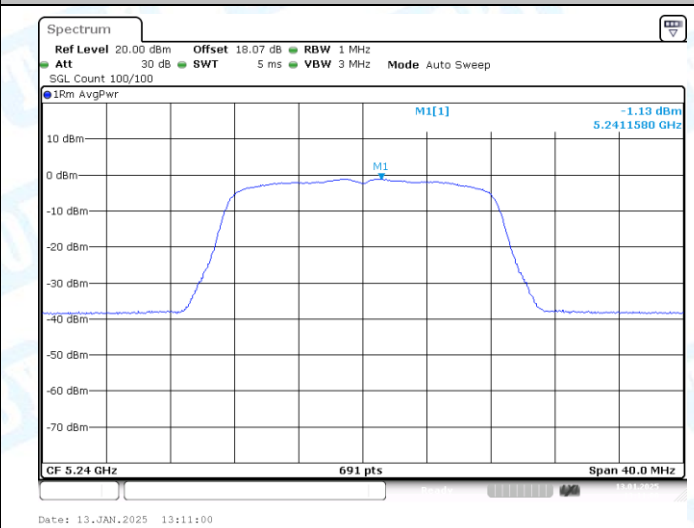
11A-CDD-Ant2-5240-PASS
