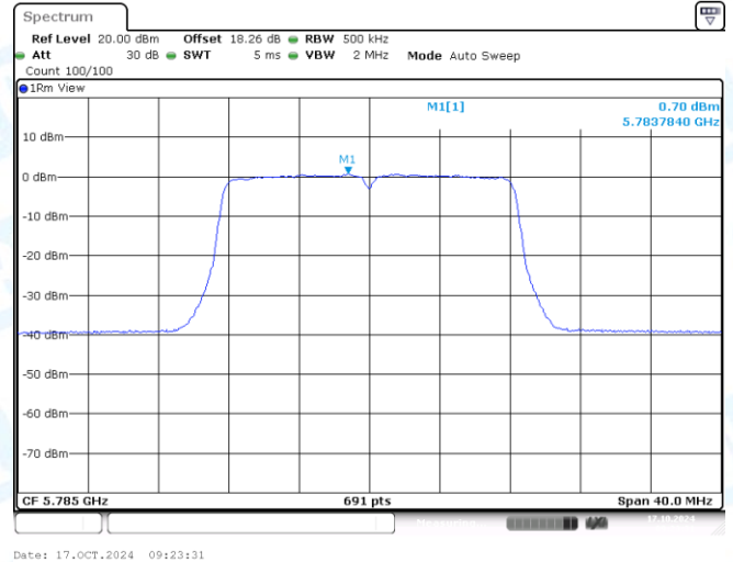
11A-CDD-Ant2-5785-PASS
