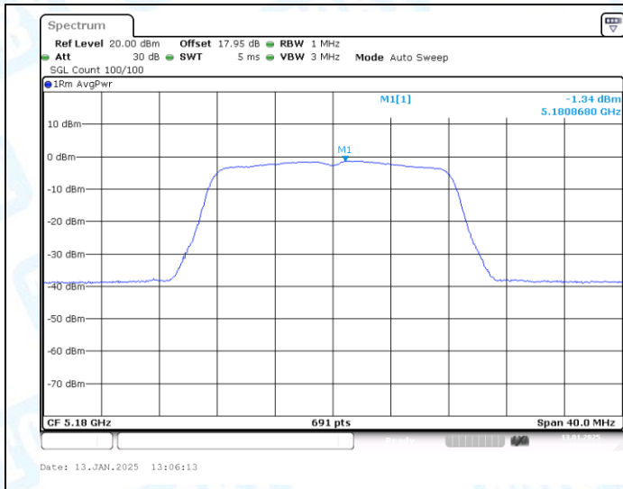
11A-CDD-Ant1-5180-PASS
