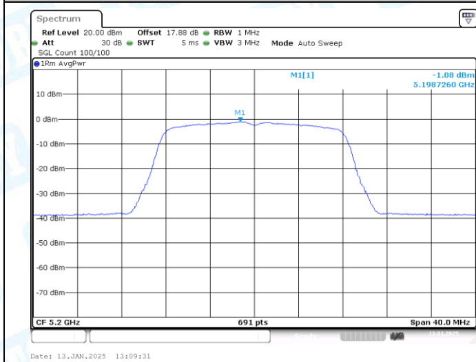
11A-CDD-Ant1-5200-PASS
