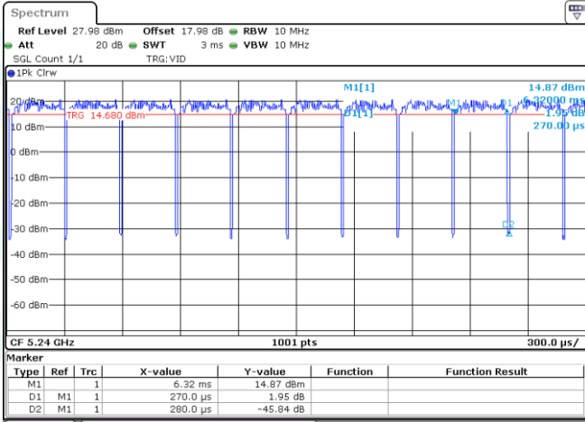
NTVN-11AX20MIMO-Ant1-5240
