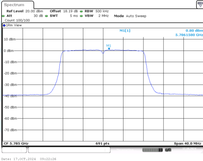
11A-CDD-Ant1-5785-PASS
