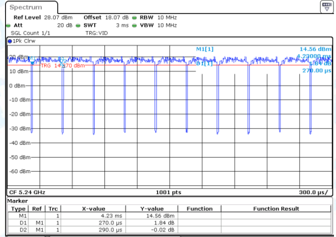
NTVN-11AX20MIMO-Ant2-5240
