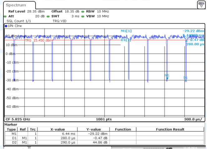
NTVN-11AX20MIMO-Ant2-5825
