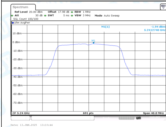
11A-CDD-Ant1-5240-PASS
