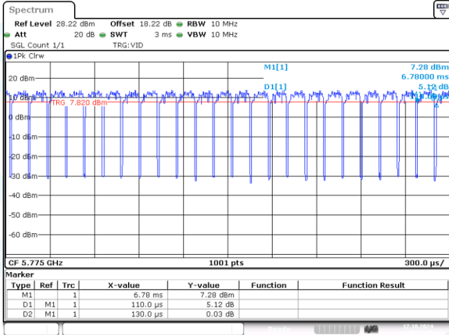
NTNV-11AX80MIMO-Ant1-5775
