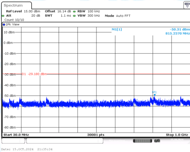
11N20MIMO-Ant1-2462-30~1000-PASS
