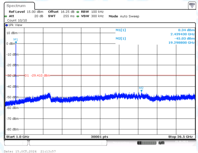
11G-CDD-Ant2-2437-1000~26500-PASS
