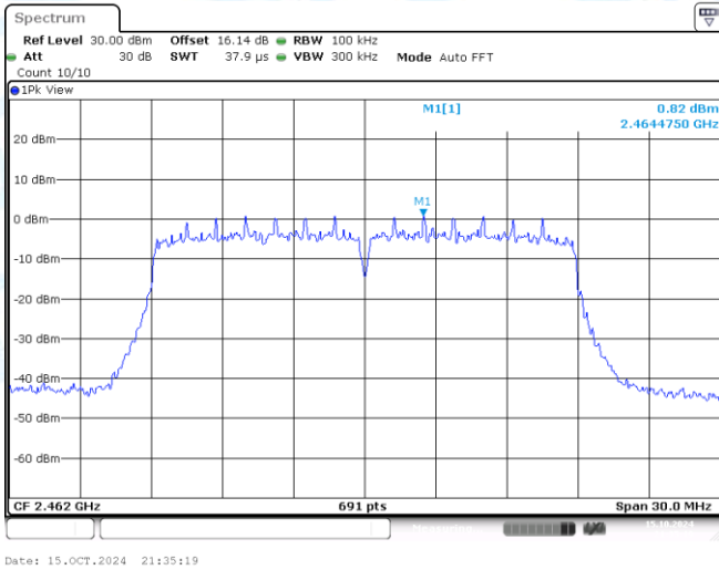
11N20MIMO-Ant1-2462-0~Reference-PASS
