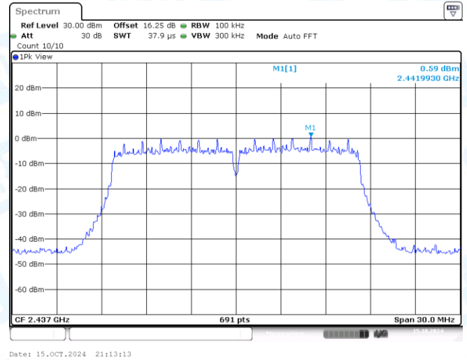
11G-CDD-Ant2-2437-0~Reference-PASS
