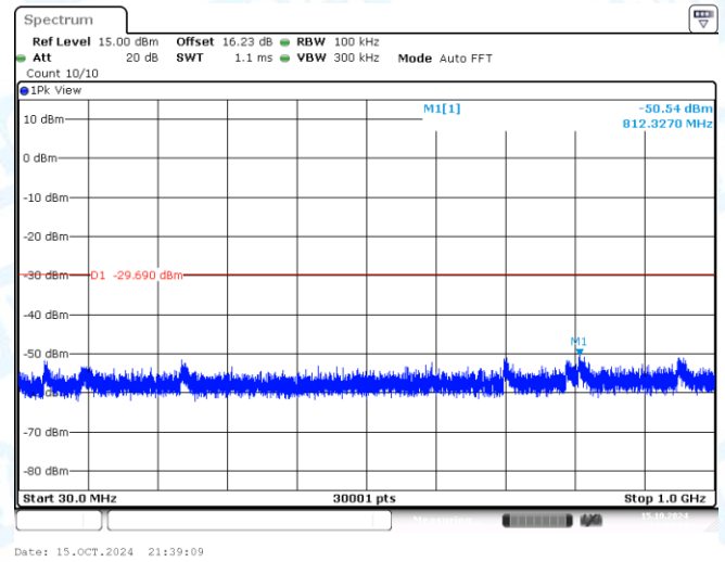
11N20MIMO-Ant2-2462-30~1000-PASS
