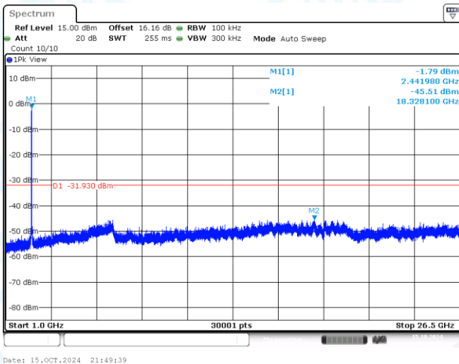
11N40MIMO-Ant1-2437-1000~26500-PASS
