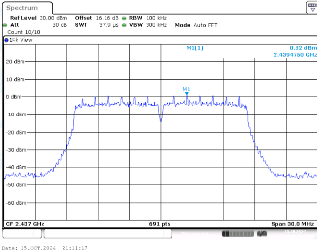
11G-CDD-Ant1-2437-0~Reference-PASS
