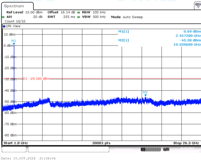
11N20MIMO-Ant1-2462-1000~26500-PASS
