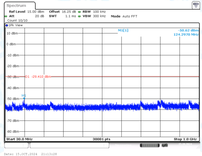
11G-CDD-Ant2-2437-30~1000-PASS
