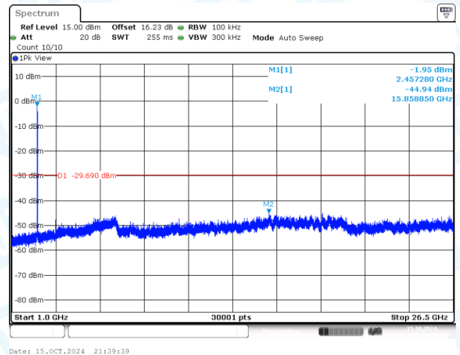
11N20MIMO-Ant2-2462-1000~26500-PASS
