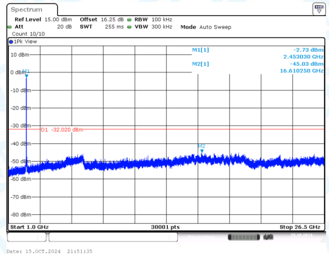
11N40MIMO-Ant2-2437-1000~26500-PASS
