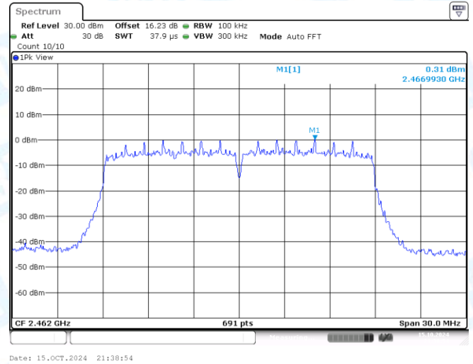
11N20MIMO-Ant2-2462-0~Reference-PASS
