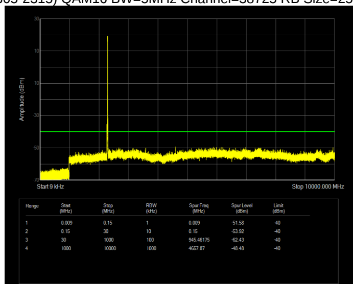
Band40(2305-2315) QAM16 BW=5MHz Channel=38725 RB Size=25 Position=#0
