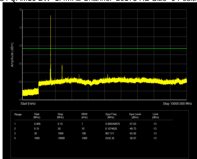
Band4 QAM16 BW=1.4MHz Channel=20175 RB Size=6 Position=#0
