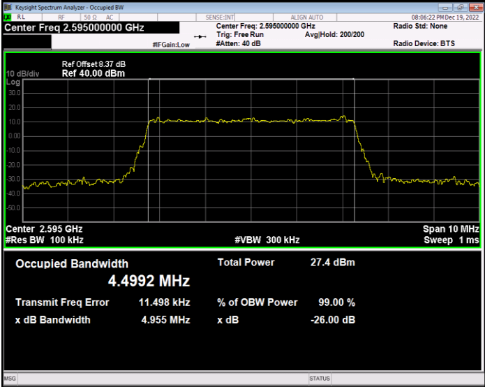
Band38 QAM16 BW=5MHz Channel=38000 RB Size=25 Position=#0
