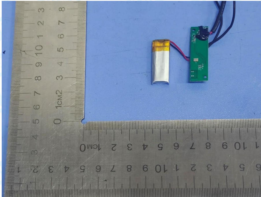
Photo 11 Appearance of PCB & Battery
