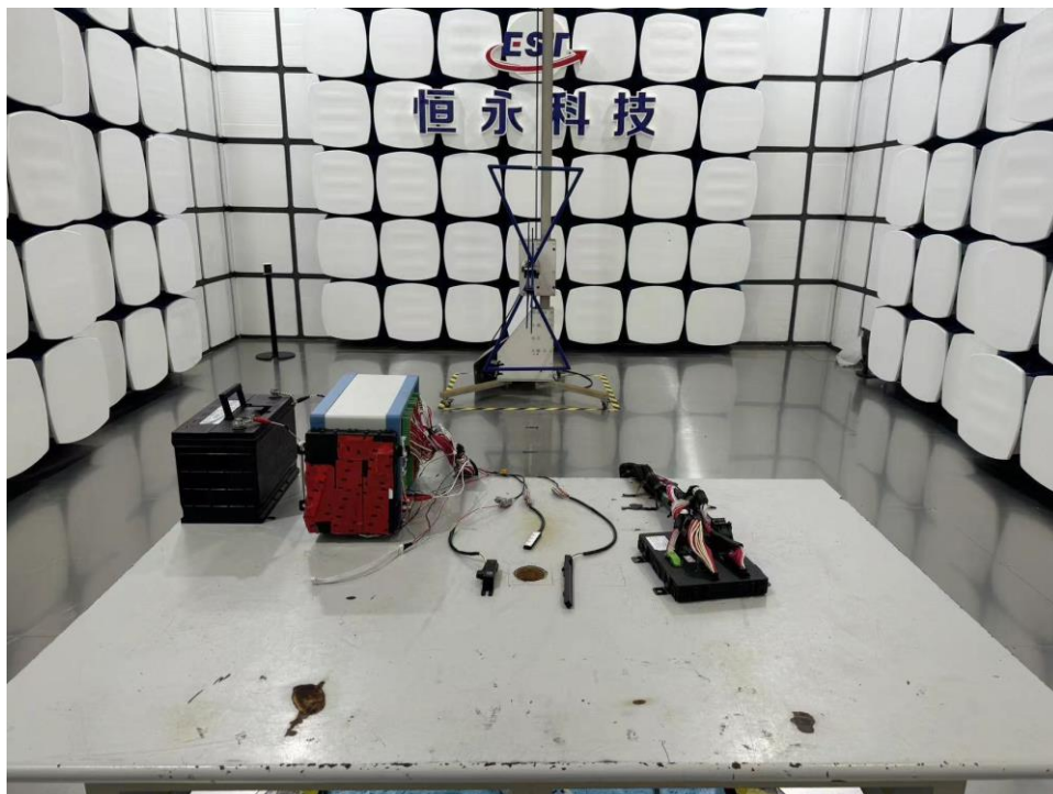
Photograph 2: Set-up photo for Radiated Spurious Emission, 30MHz - 1000MHz
