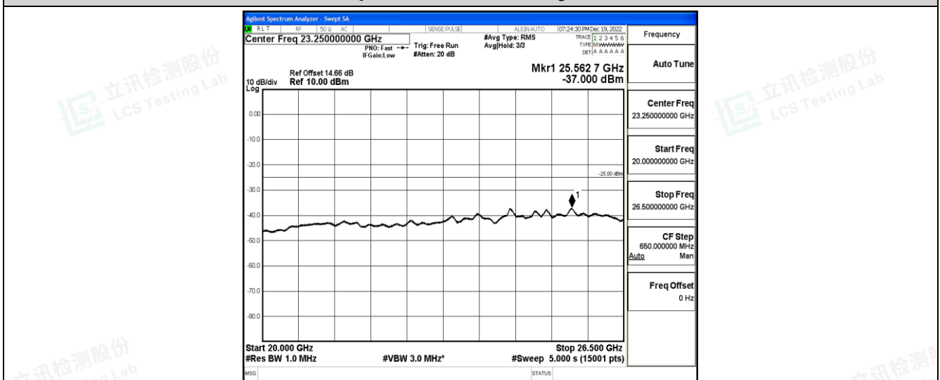
Band41-20MHz-16QAM-41490-1RB#0-Range6:20000~26500MHz
