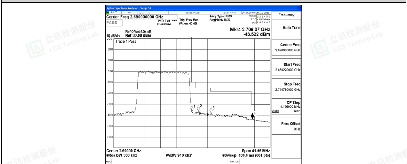
Band41-15MHz-16QAM-39725-75RB#0
