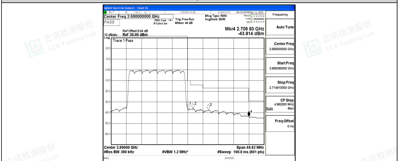
Band41-20MHz-16QAM-41490-100RB#0
