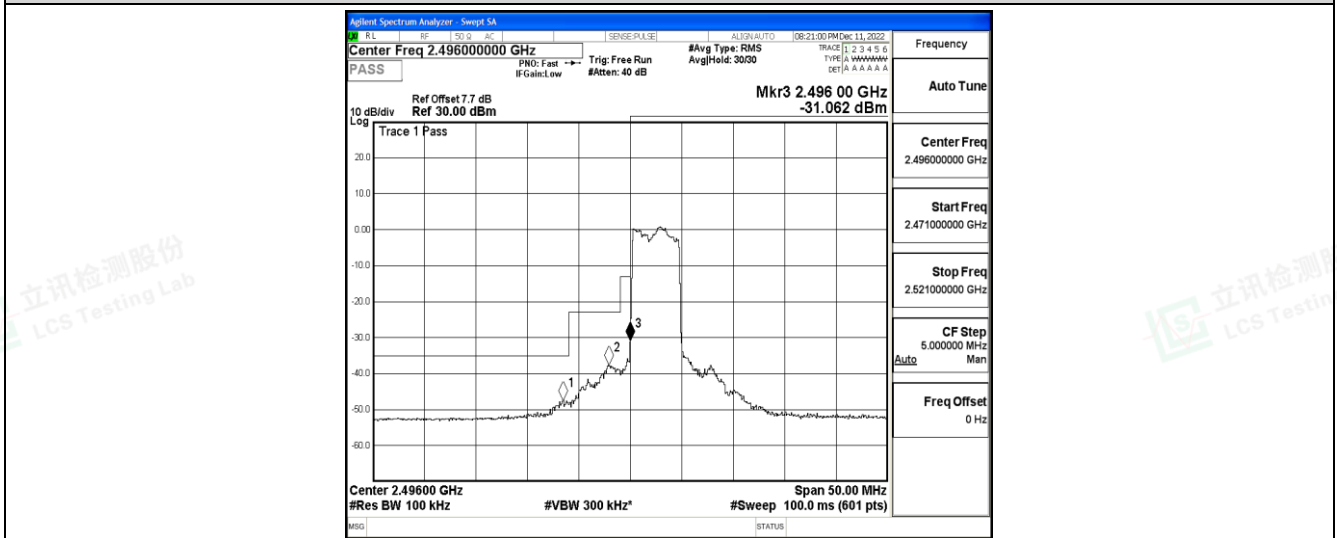
Band41-5MHz-16QAM-41565-25RB#0
