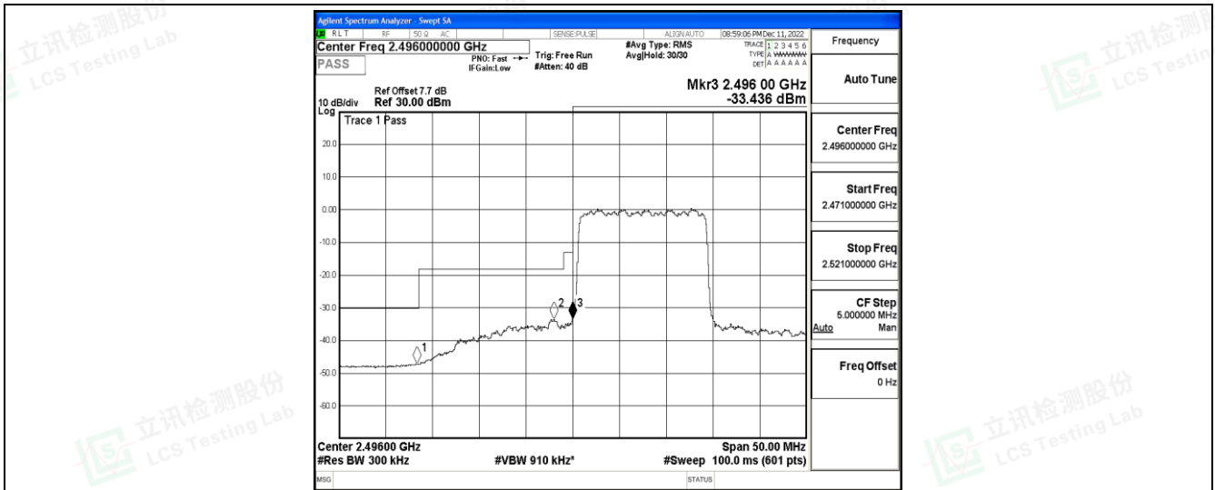
Band41-15MHz-16QAM-41515-75RB#0
