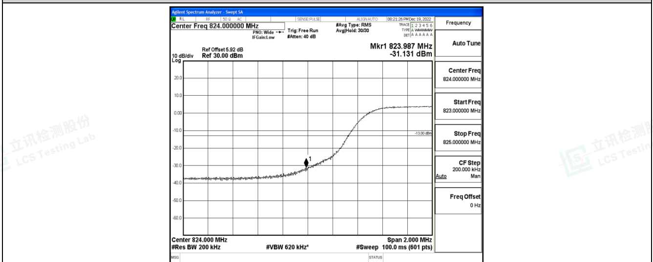
Band26-10MHz-QPSK-26990-50RB#0
