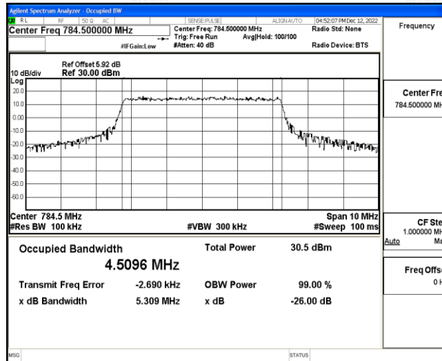
Band13-5MHz-16QAM-23205-25RB#0
