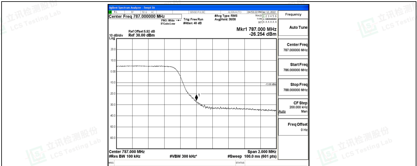
Band13-5MHz-16QAM-23205-25RB#0
