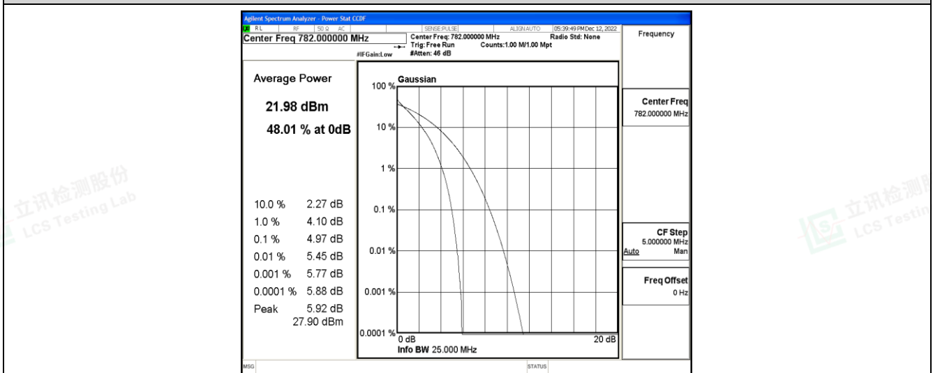
Band13-10MHz-16QAM-23230-50RB#0
