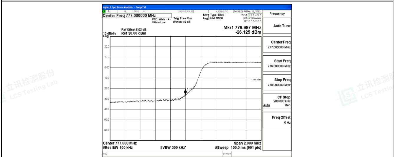
Band13-5MHz-16QAM-23255-25RB#0
