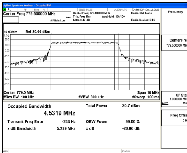
Band13-5MHz-QPSK-23230-25RB#0
