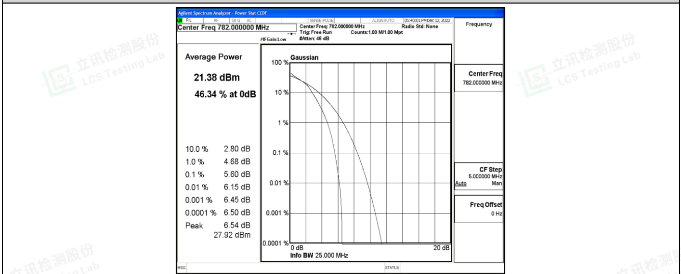
Band13-10MHz-16QAM-23230-50RB#0
