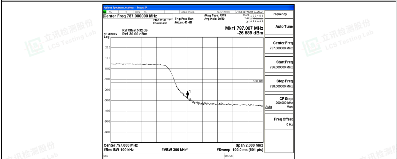
Band13-10MHz-QPSK-23230-50RB#0
