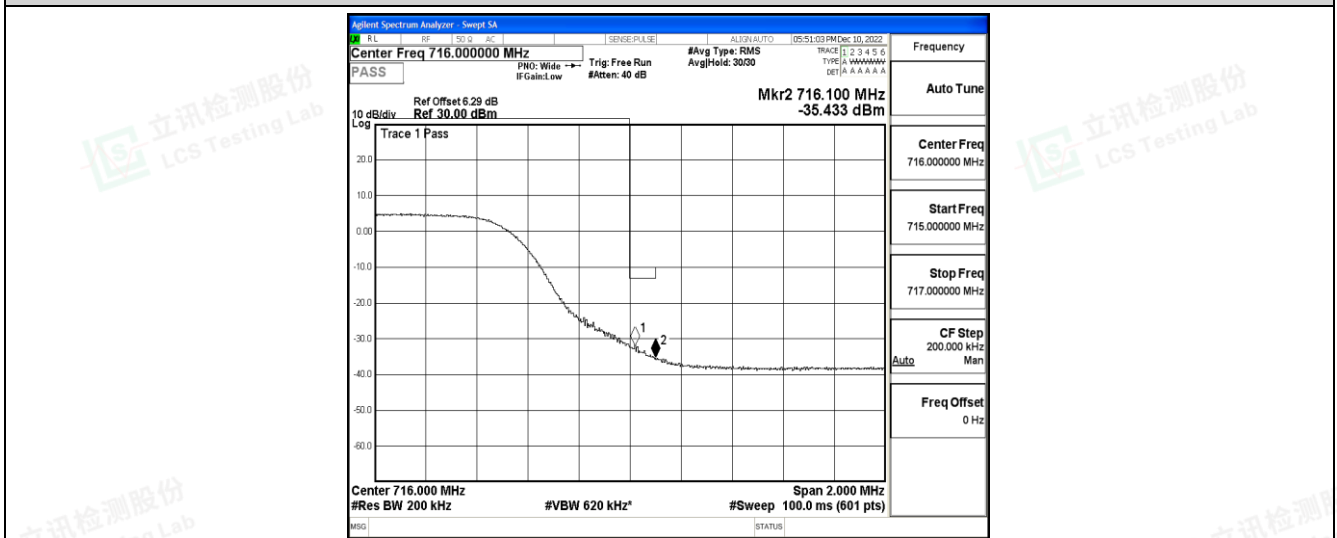
Band12-10MHz-16QAM-23130-50RB#0
