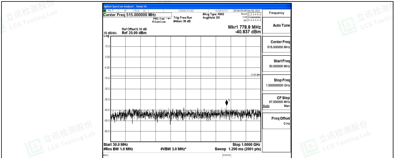
Band4-10MHz-16QAM-20000-1RB#0-Range4:1000~10000MHz
