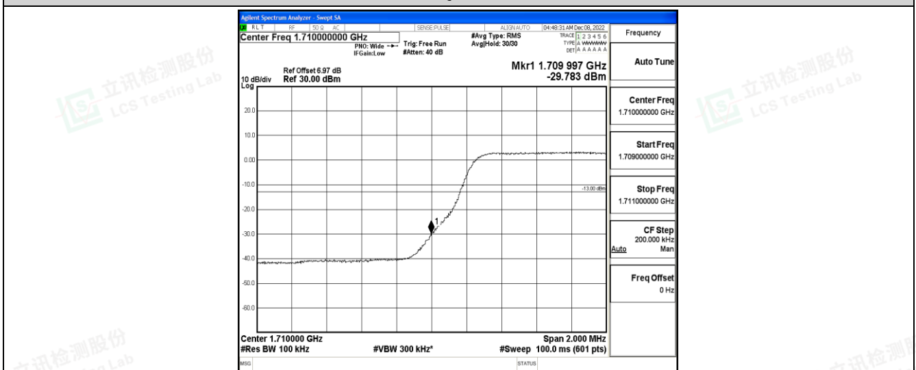
Band4-5MHz-16QAM-20375-25RB#0
