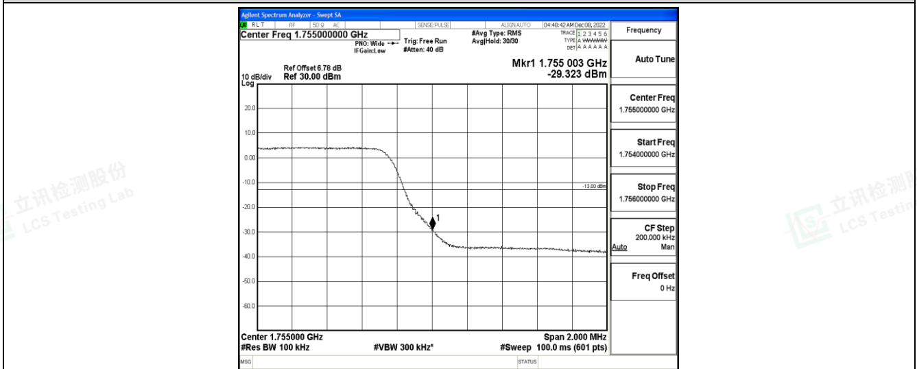
Band4-5MHz-16QAM-19975-25RB#0
