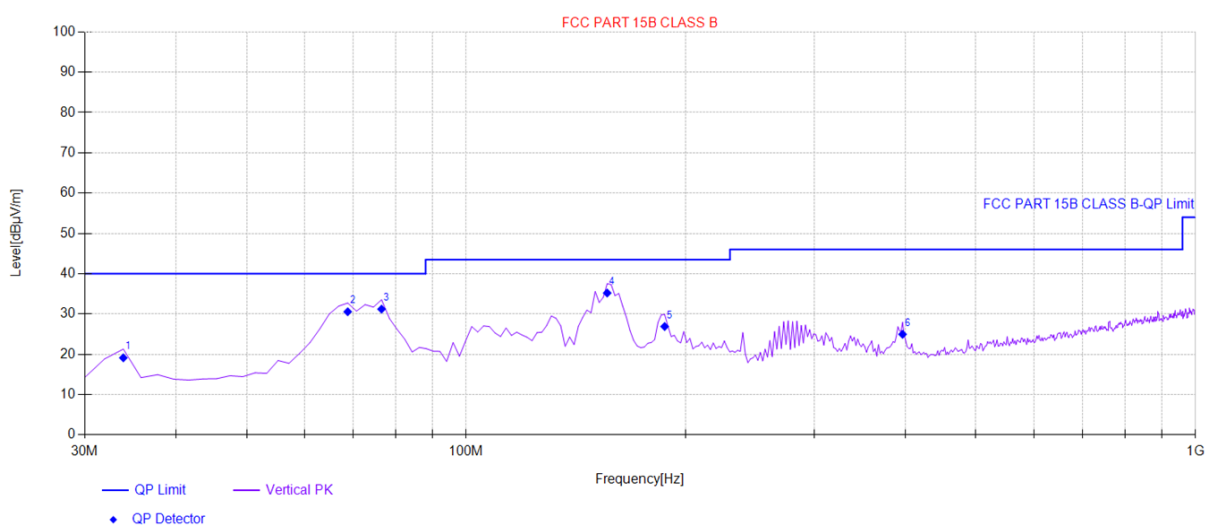
Test plot for Vertical: GFSK(2402MHz)
