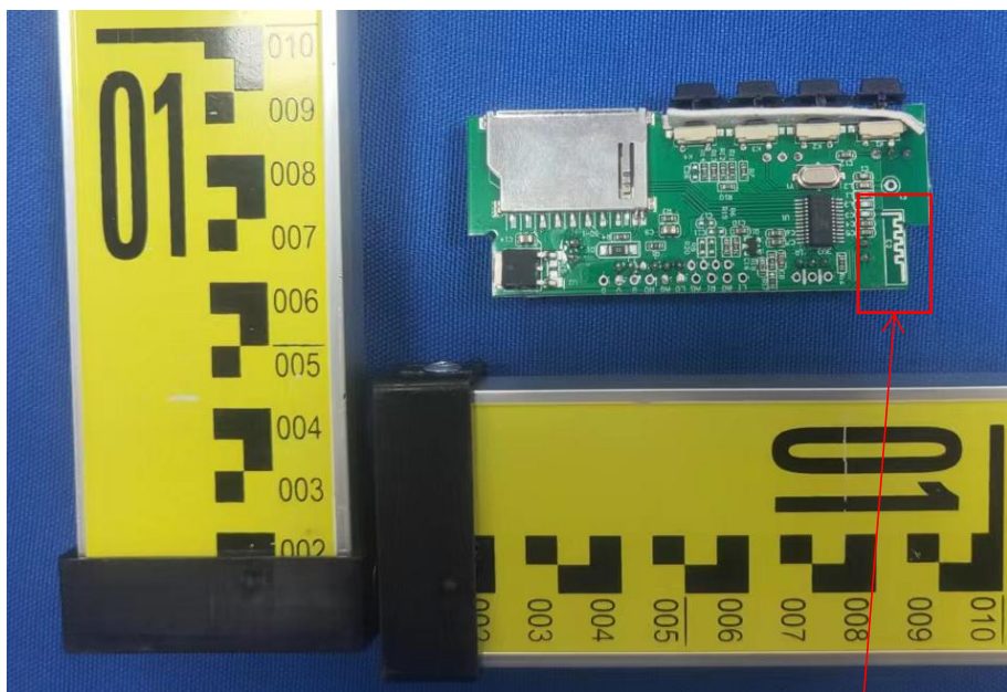
BT antenna
