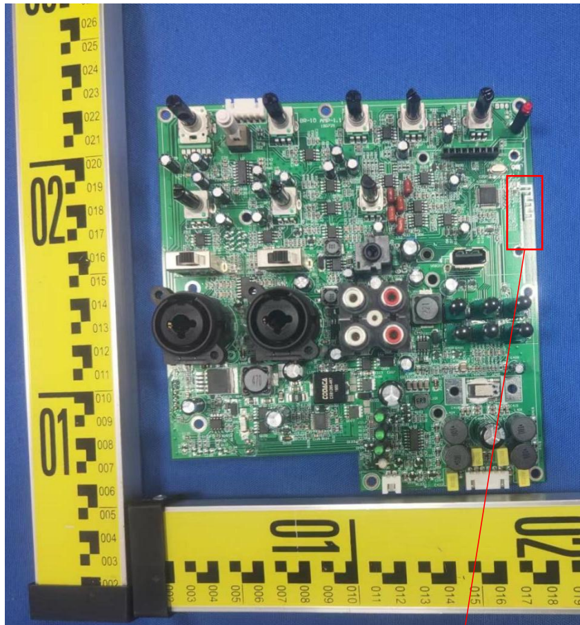
BT antenna
