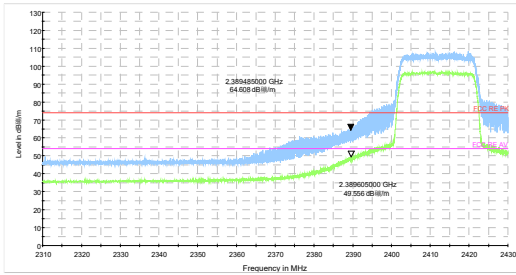
802.11ax HE20 242-Tone-CH1 Peak+ Average
