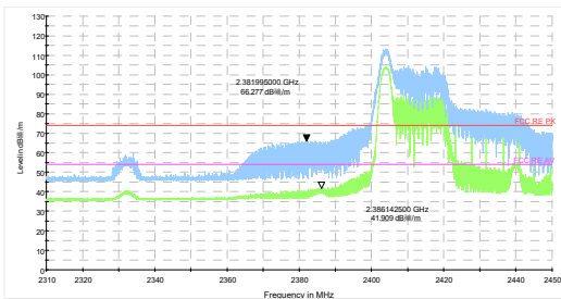
802.11ax HE40 26-Tone-CH3 Peak+ Average
