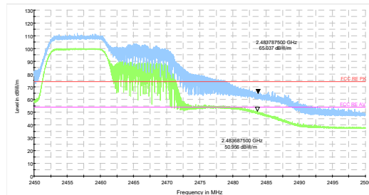
802.11ax HE20 106-Tone-CH11 Peak+ Average
