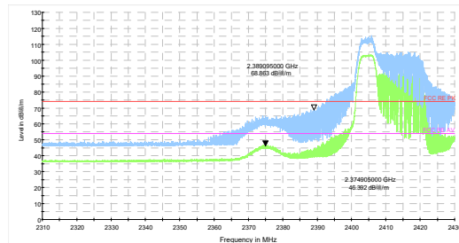
802.11ax HE20 52-Tone-CH1 Peak+ Average
