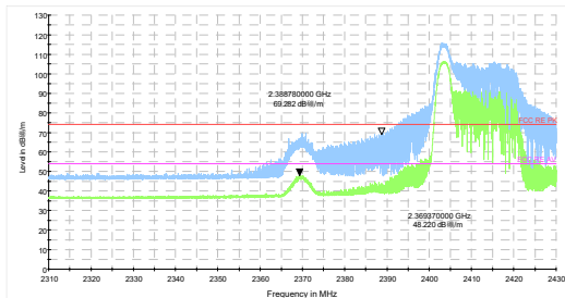
802.11ax HE20 26-Tone-CH1 Peak+ Average
