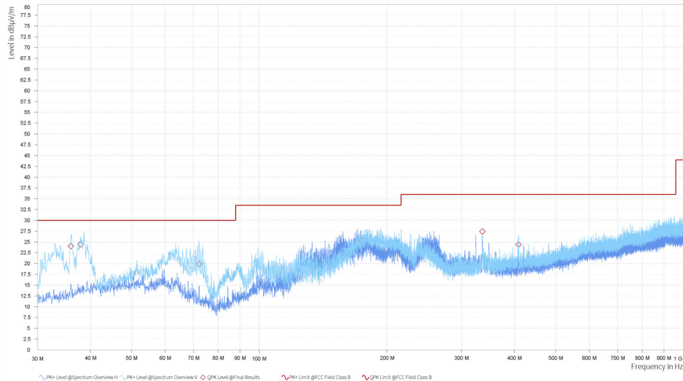
Radiates Emission from 30MHz to 1GHz
