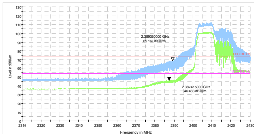
802.11ax HE20 106-Tone-CH1 Peak+ Average
