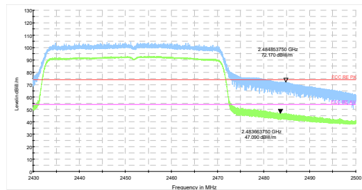
802.11ax HE40 484-Tone-CH9 Peak+ Average
