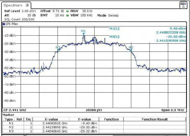
8DPSK_3-DH5_Channel 39
