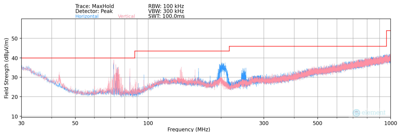
Plot 7-4. Radiated Measurements at 3-meters – Below 1GHz
