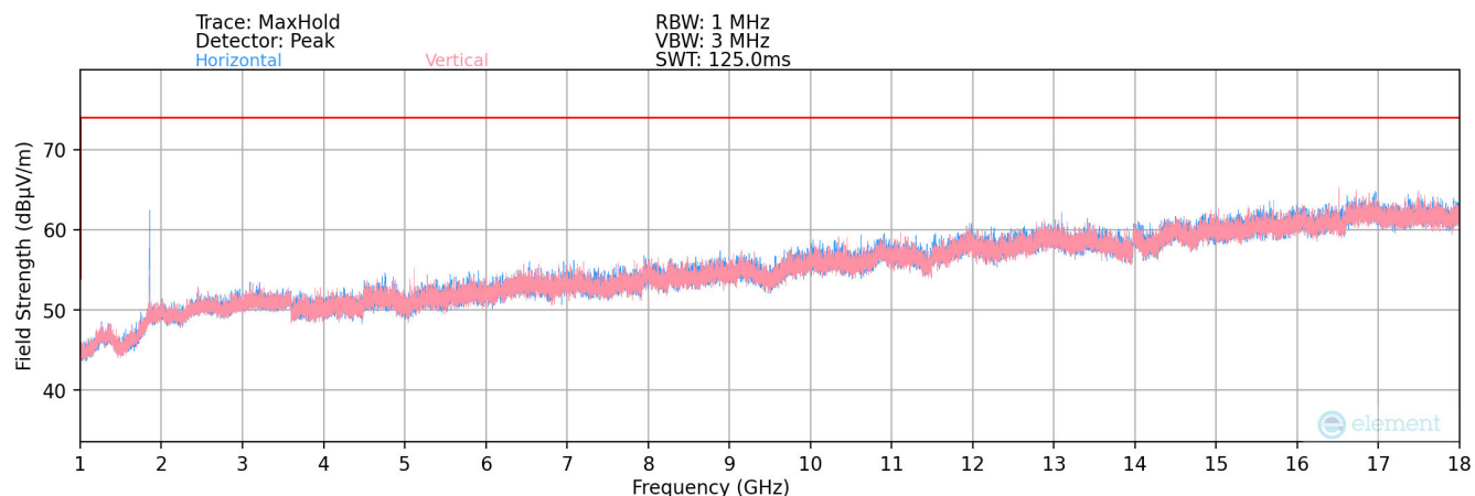
Plot 7-5. Radiated Measurements at 3-meters – Above 1GHz
