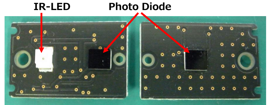
Sensor boards (Back)
