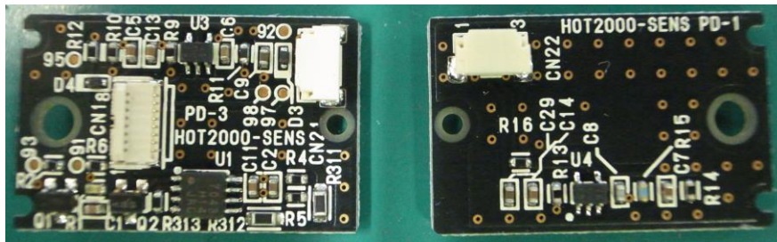
Sensor boards (Front)
