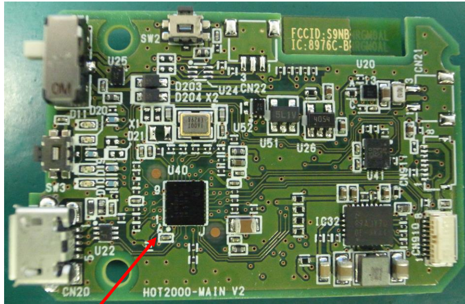
Main board (Front)
