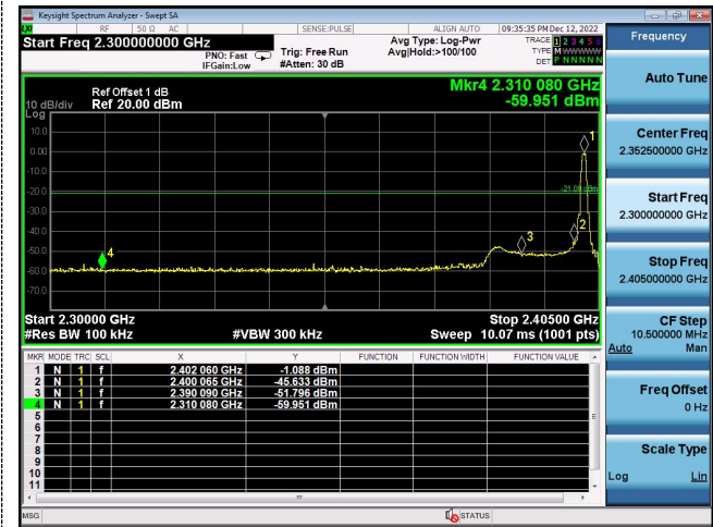
Left bandedge
