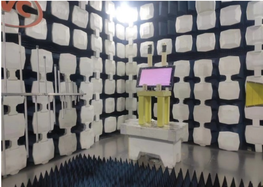
Description: Test Setup
