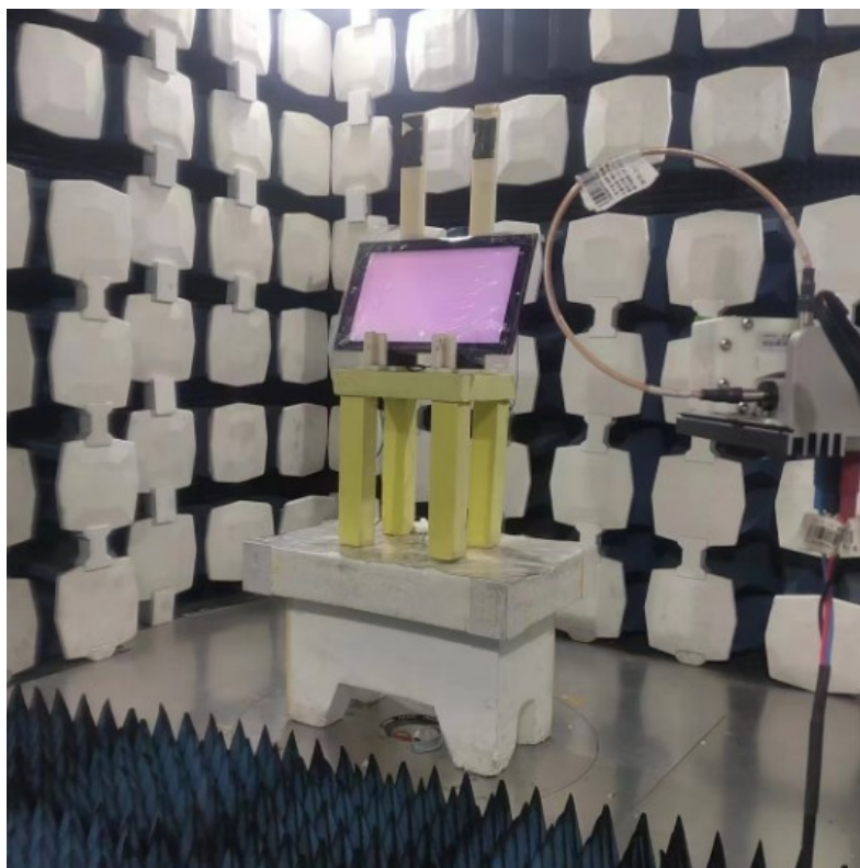
Description: Test Setup
