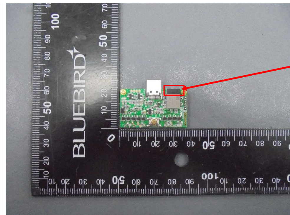
Chip Antenna
