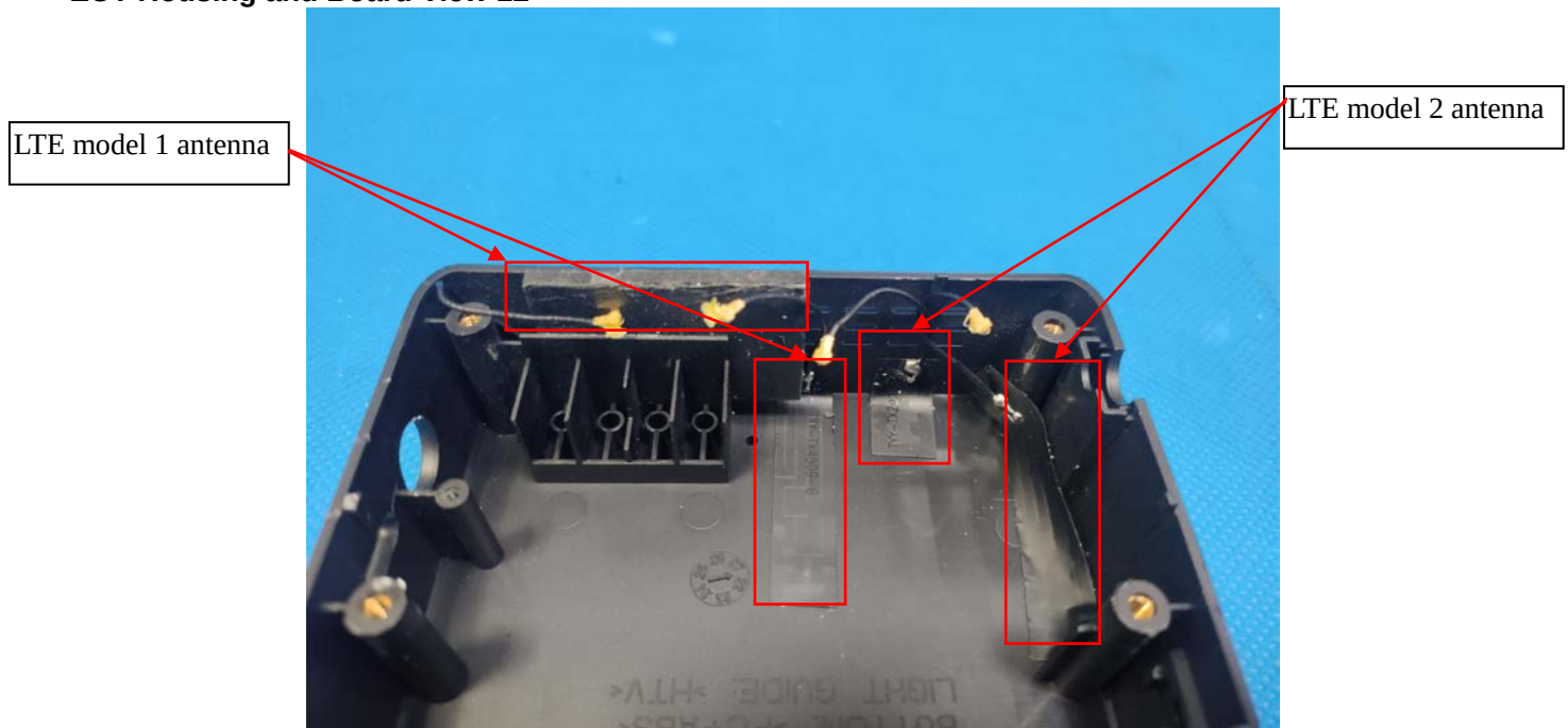
EUT Housing and Board View 12
