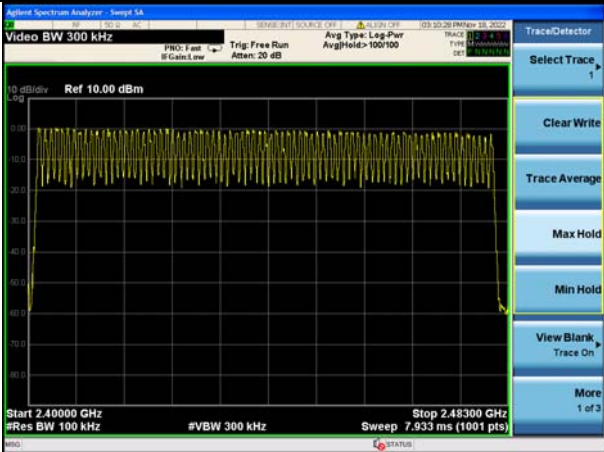
GFSK Modulation
