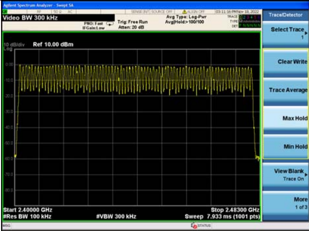
8DPSK Modulation
