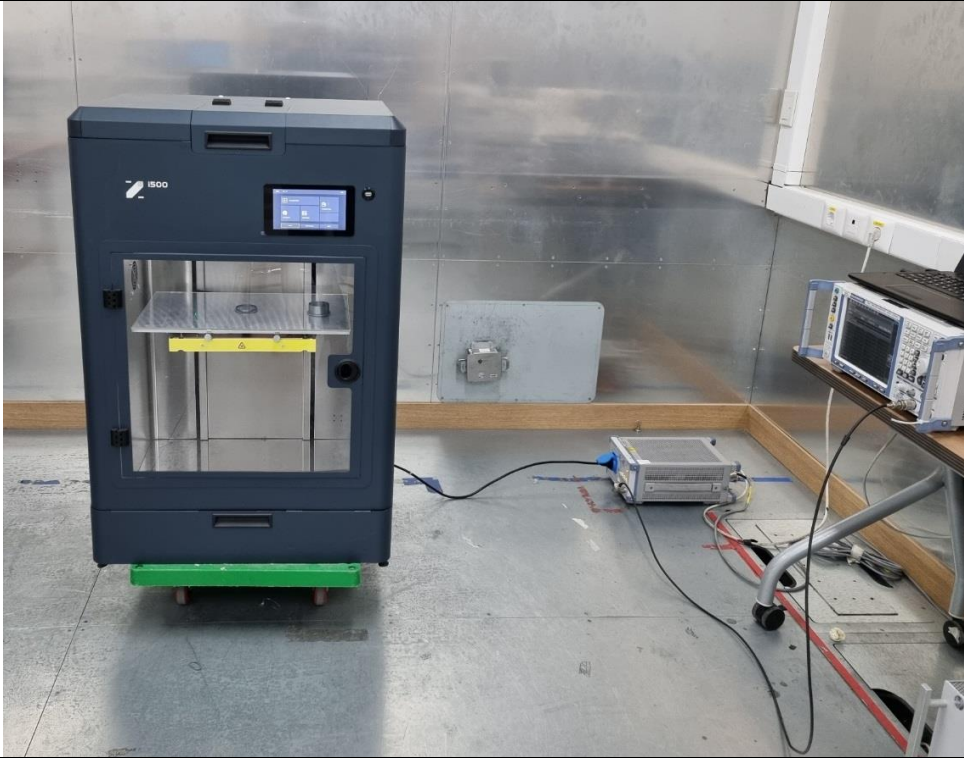
Power Line Conducted Emission (Side)
